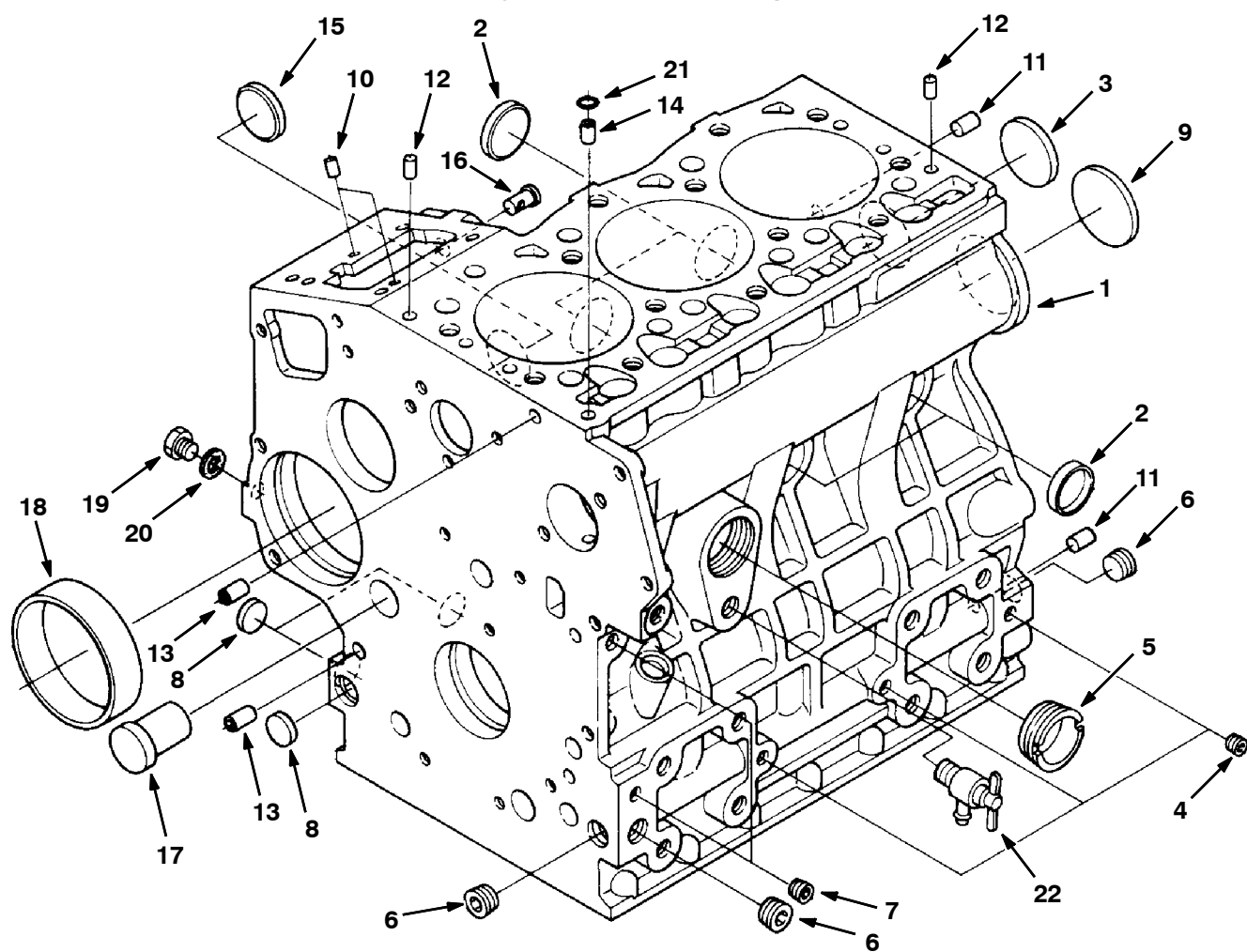
Fig. 1 - Crankcase Group
