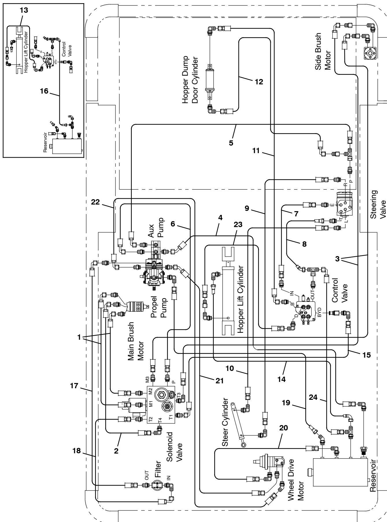
Fig. 37 - Hydraulic Hose Group
