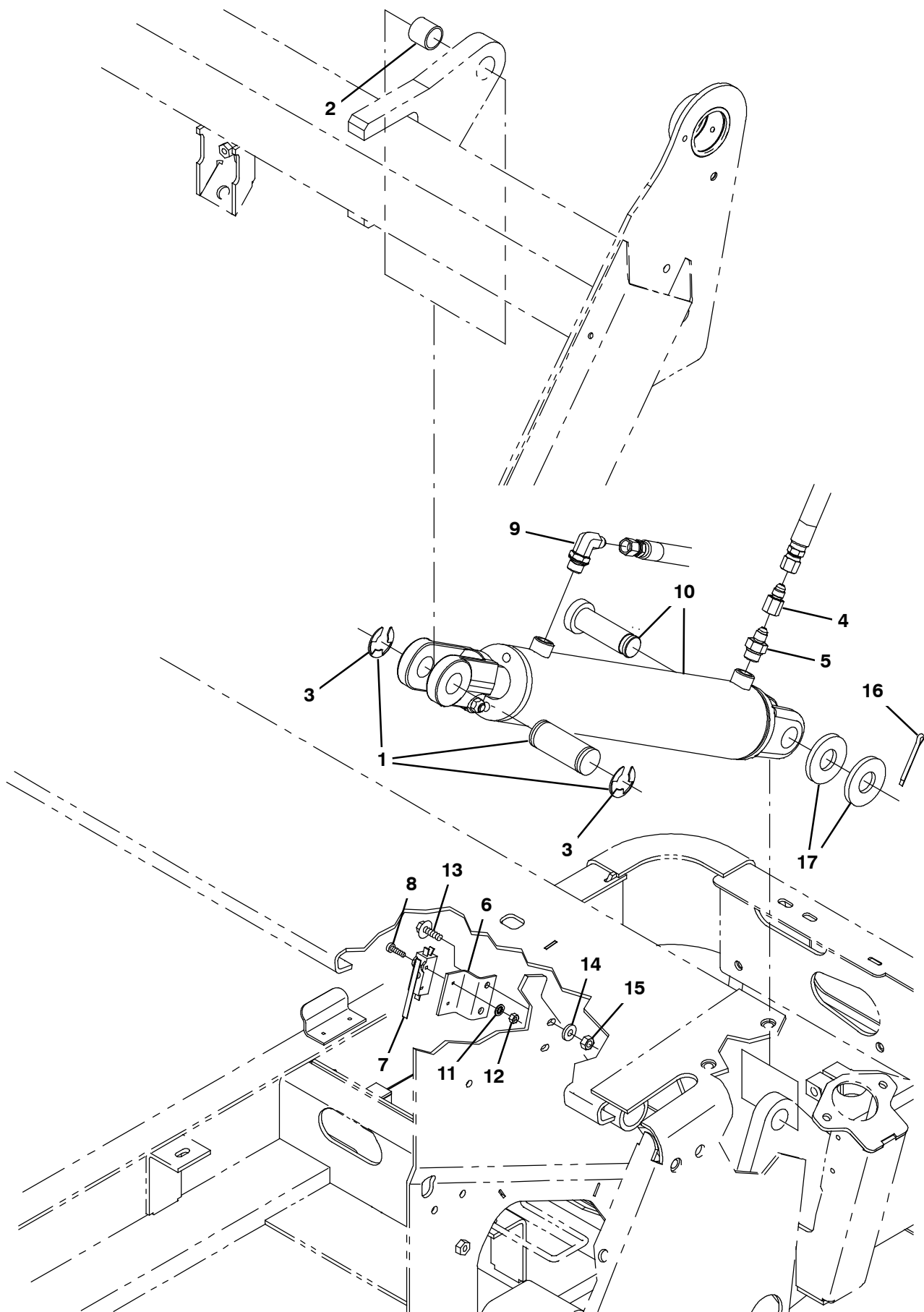
Fig. 28 - Hopper Lift Cylinder Group
