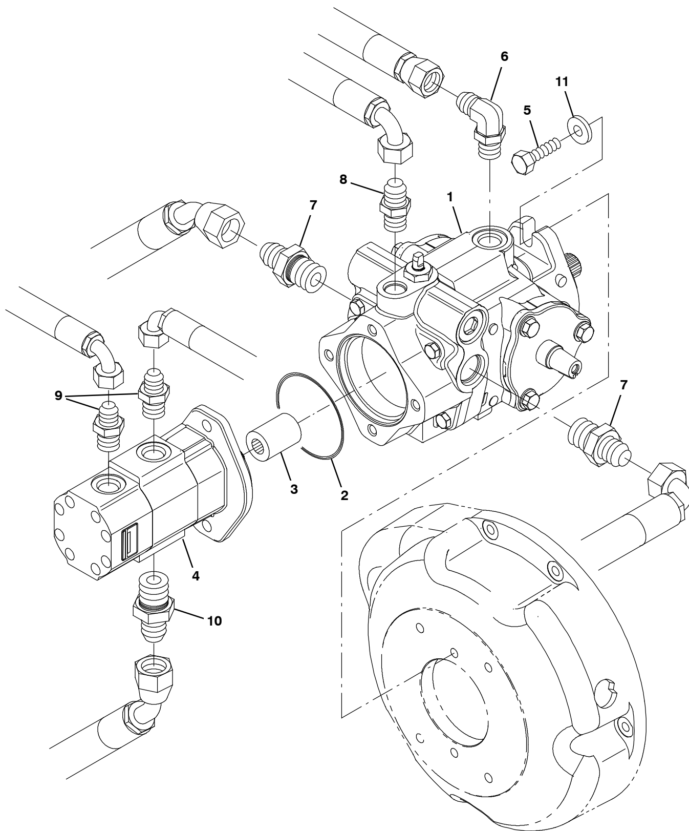
Fig. 38 - Hydraulic Pumps Group
