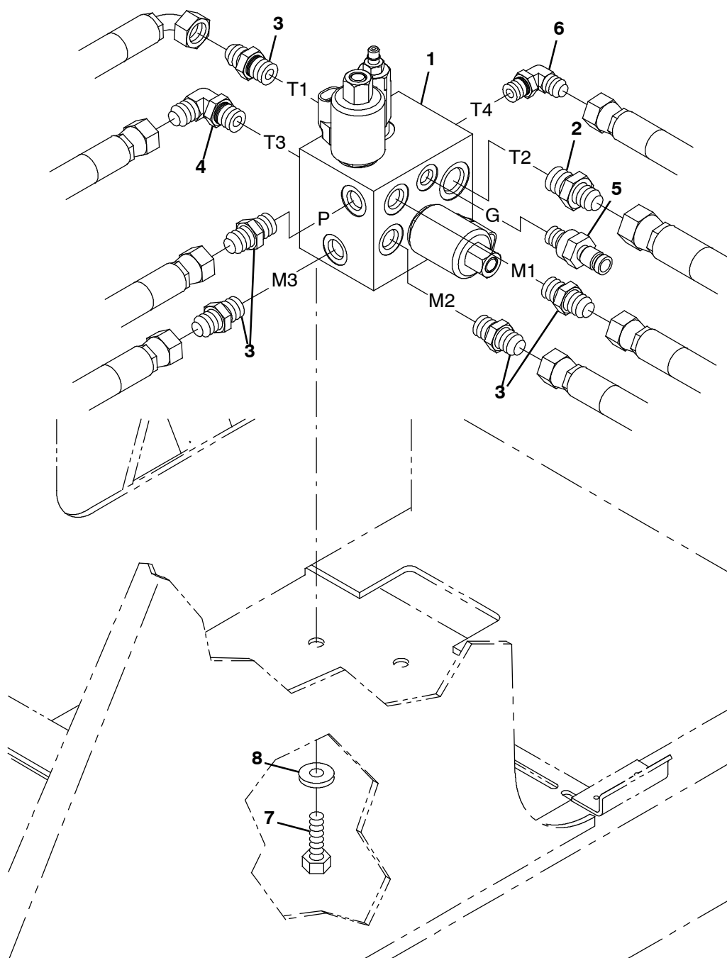
Fig. 41 - Hydraulic Solenoid Valve Group
