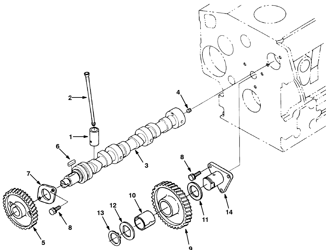
Fig. 13 - Camshaft Group
