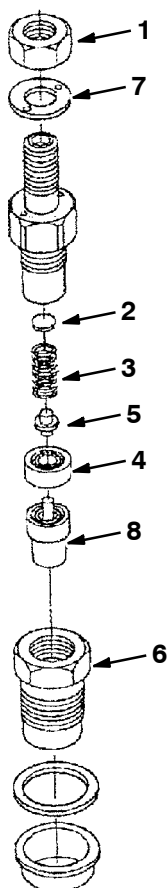
Fig. 21 - Nozzle Holder Breakdown
