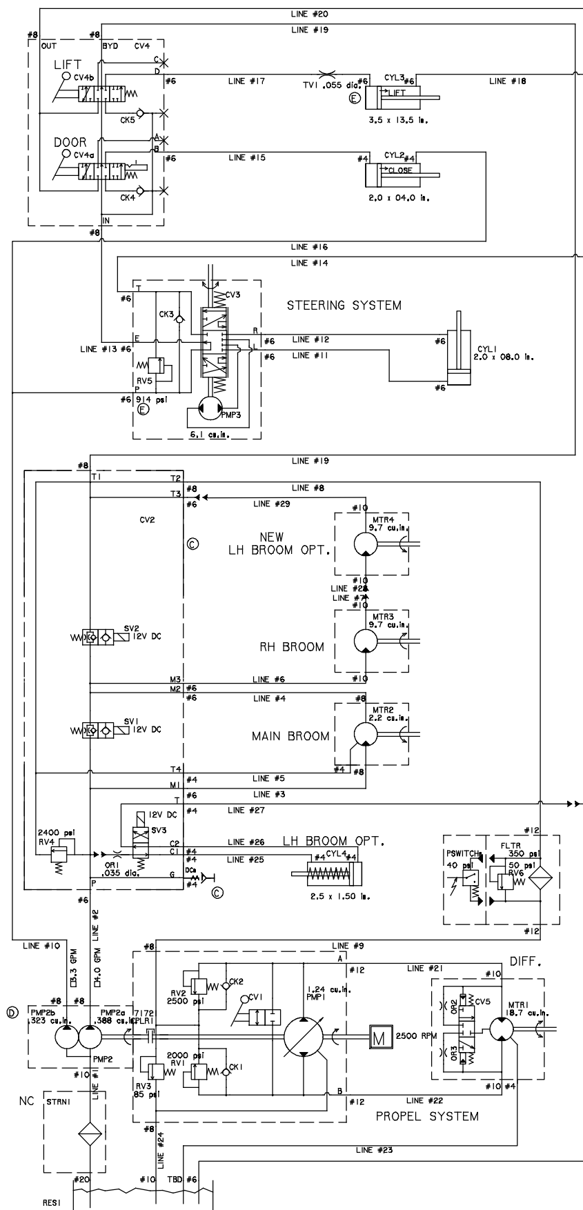
Fig. 36 - Hydraulic Schematic
