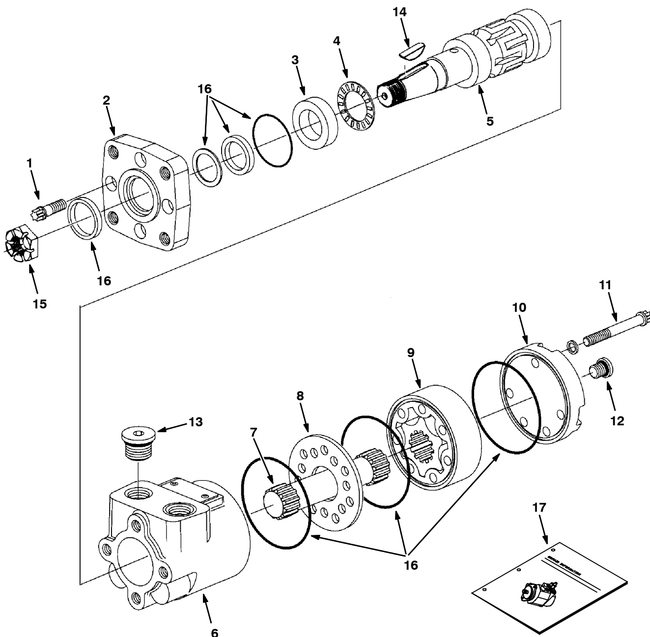
Fig. 3 - Hydraulic Gear Motor Breakdown, 361021
