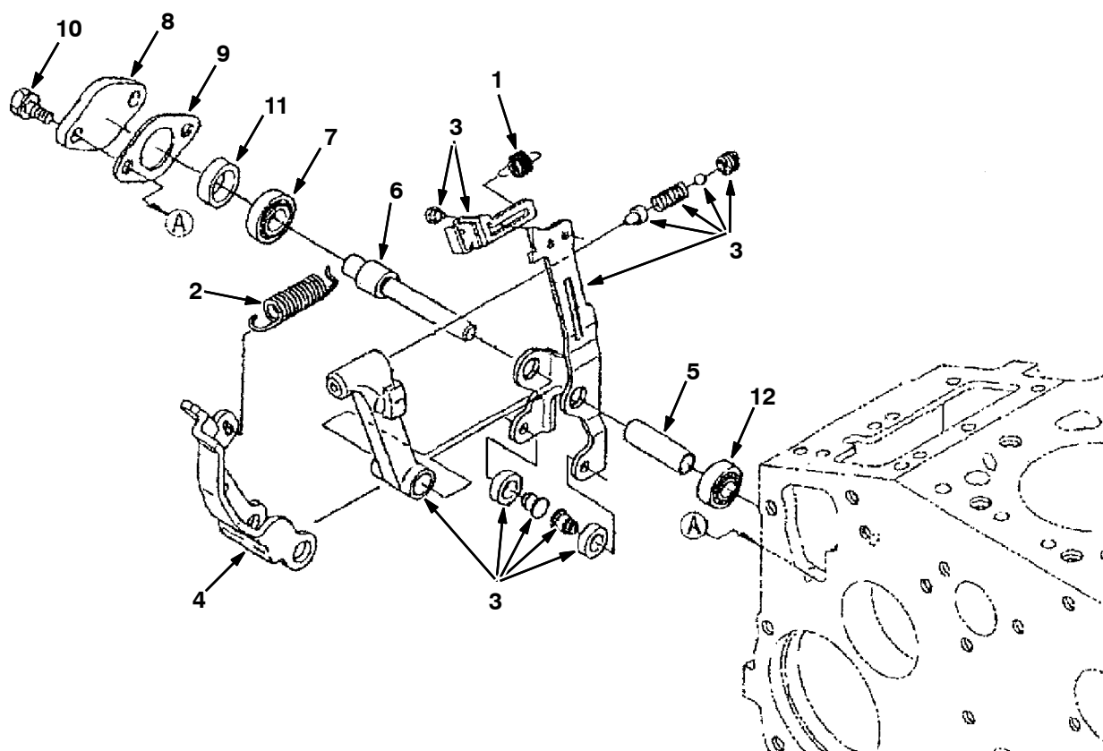
Fig. 18 - Governor Group
