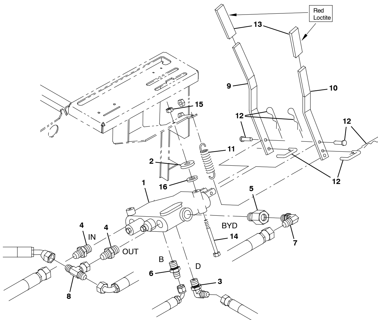
Fig. 40 - Hydraulic Control Valve Group
