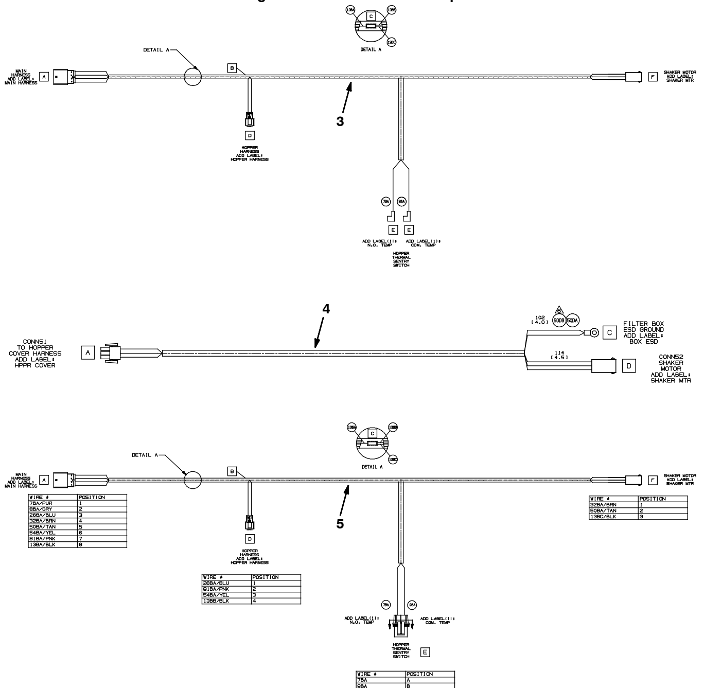
Fig. 43 - Wire Harness Group
