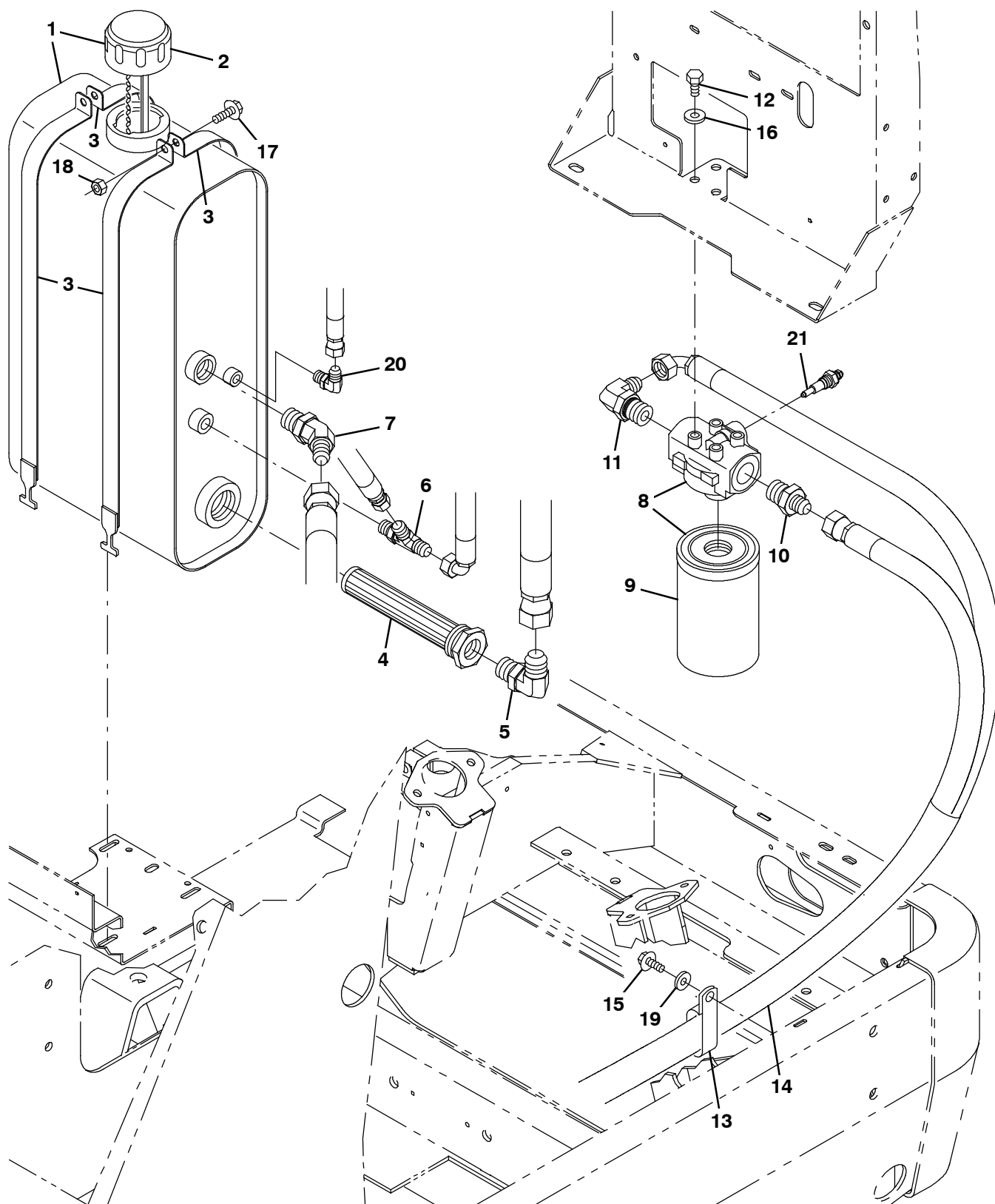
Fig. 39 - Hydraulic Reservoir Group
