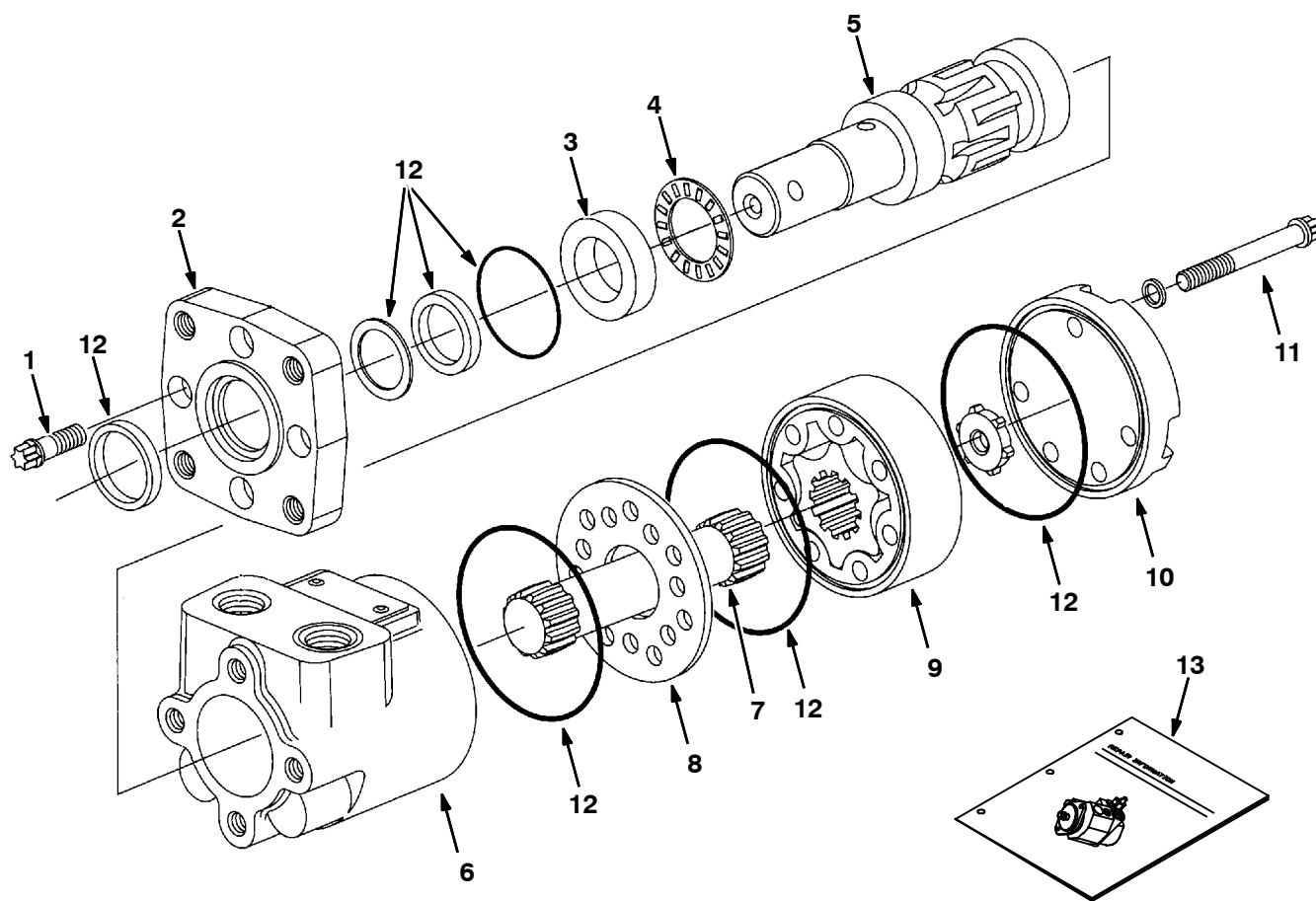
Fig. 2 - Hydraulic Gear Motor Breakdown, 361014
