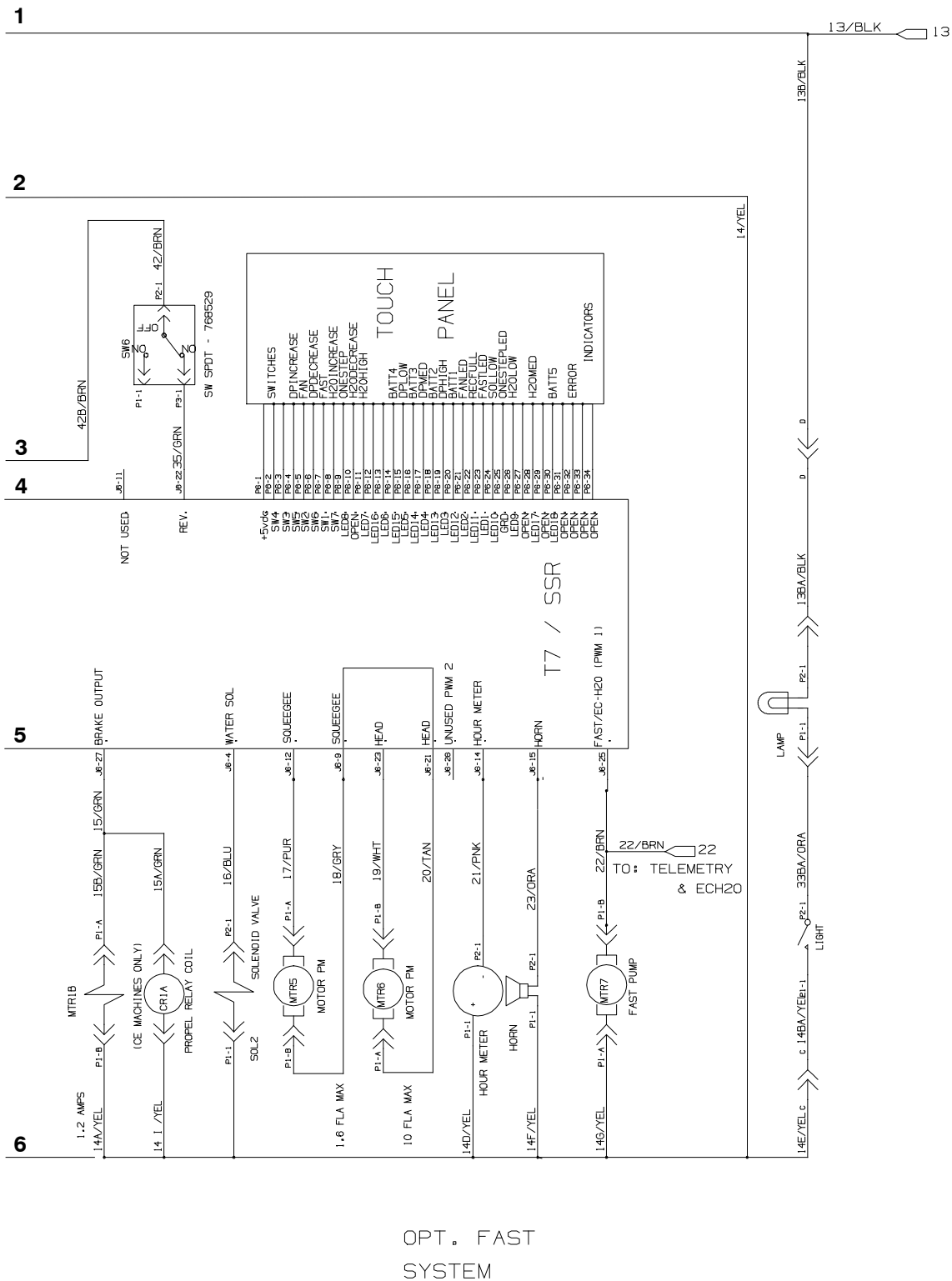
Fig. 33 - Electrical Schematic, Standard, FaST & ec-H2O Models (S/N 12695- )
