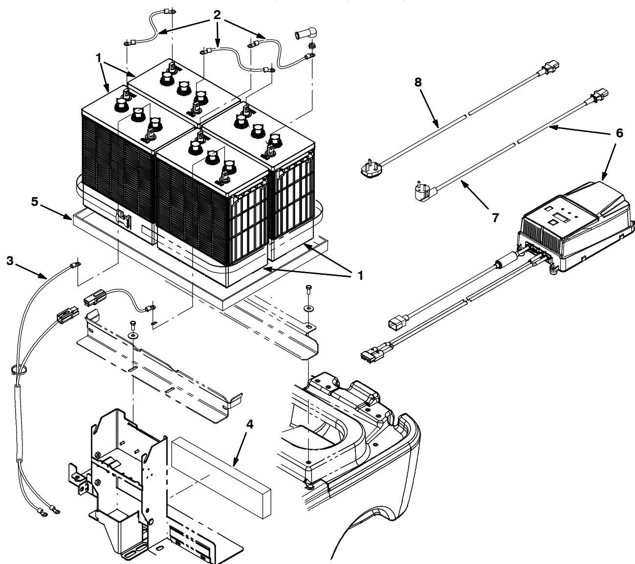
Fig. 11 - Battery and Charger Group 360Ah/5H
