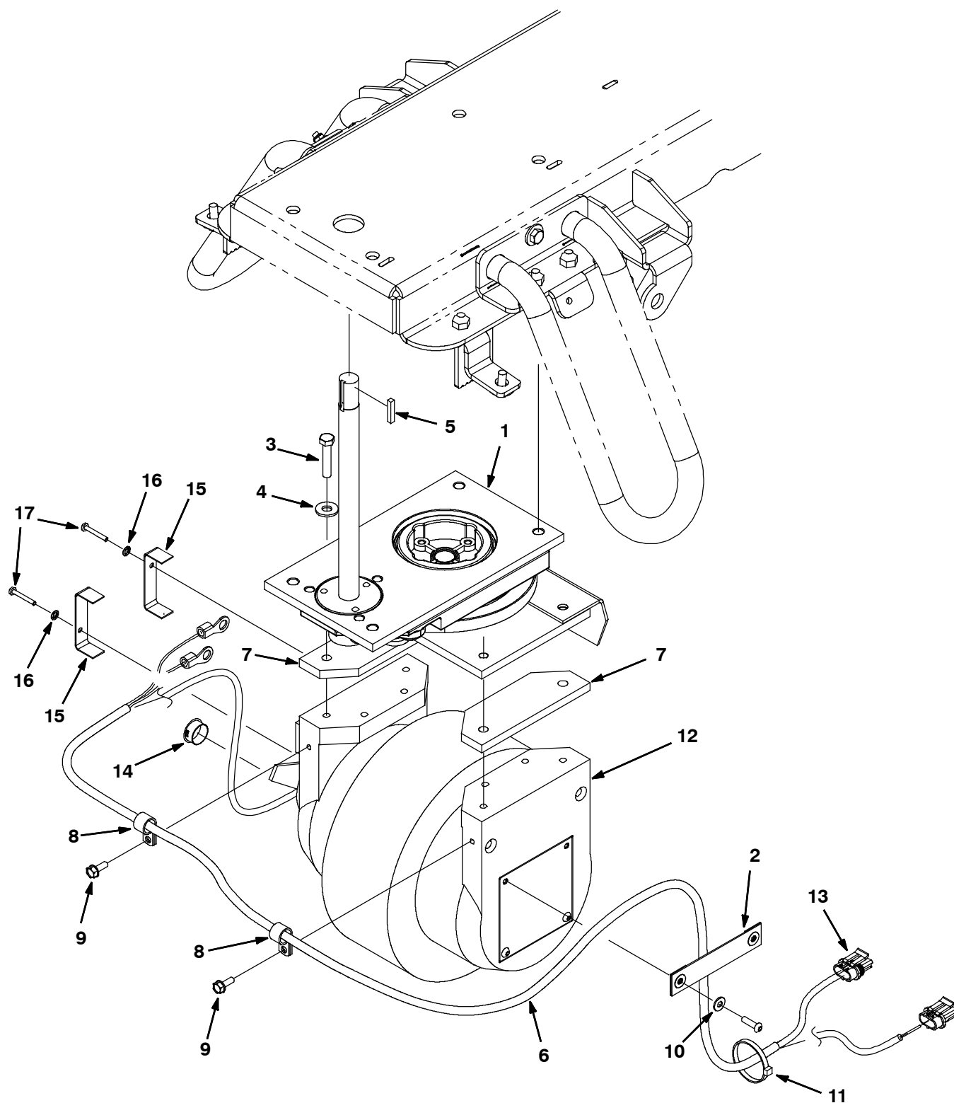
Fig. 9 - Front Drive Wheel Group
