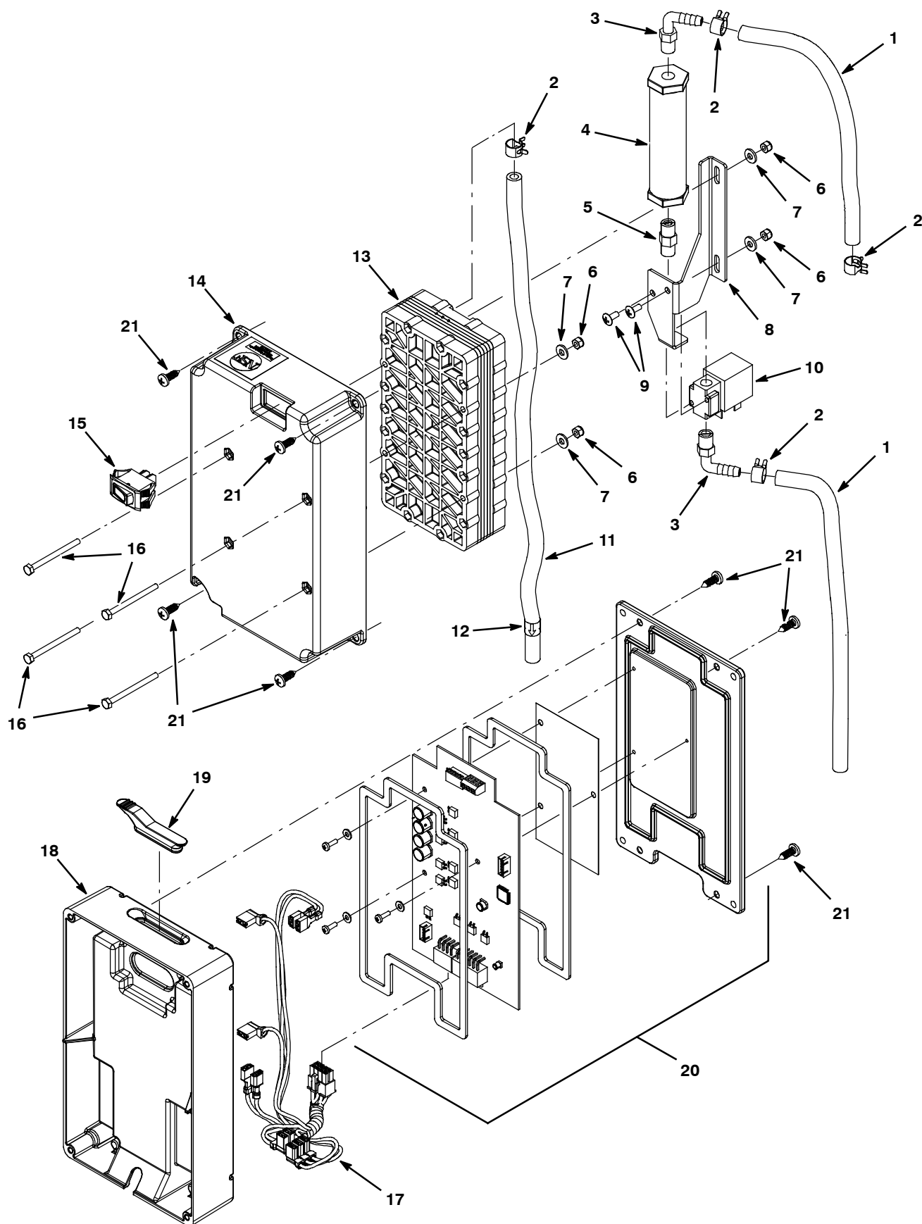
Fig. 4 - ec-H2O Module Assembly Breakdown, 9007970 (S/N 10000-10999)
