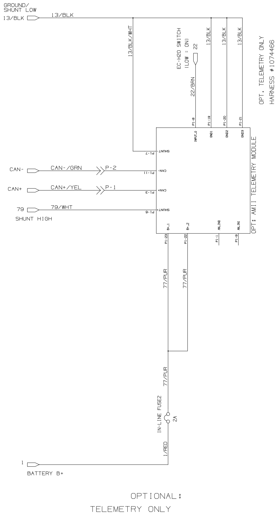
Fig. 33 - Electrical Schematic, Standard, FaST & ec-H2O Models (S/N 12695- )
