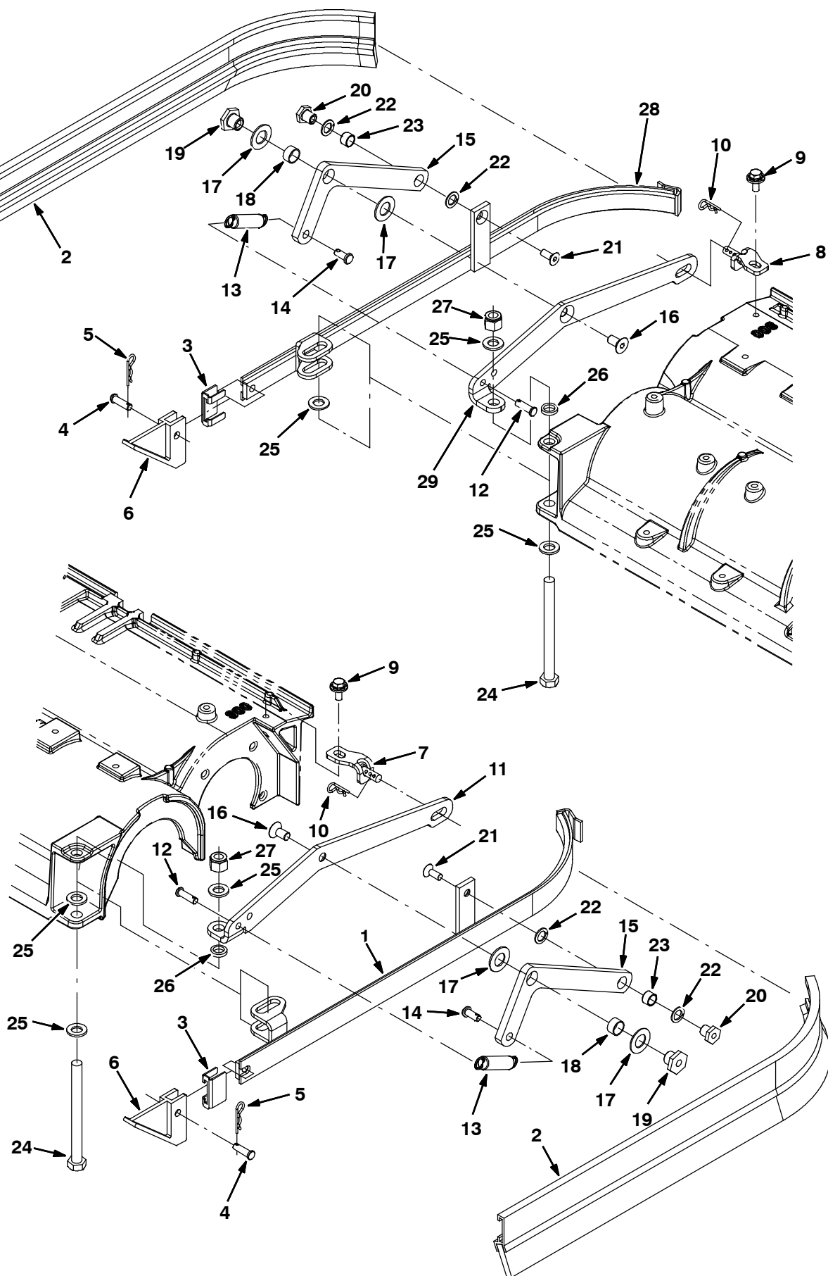
Fig. 21 - Cylindrical Scrub Head Squeegee Group
