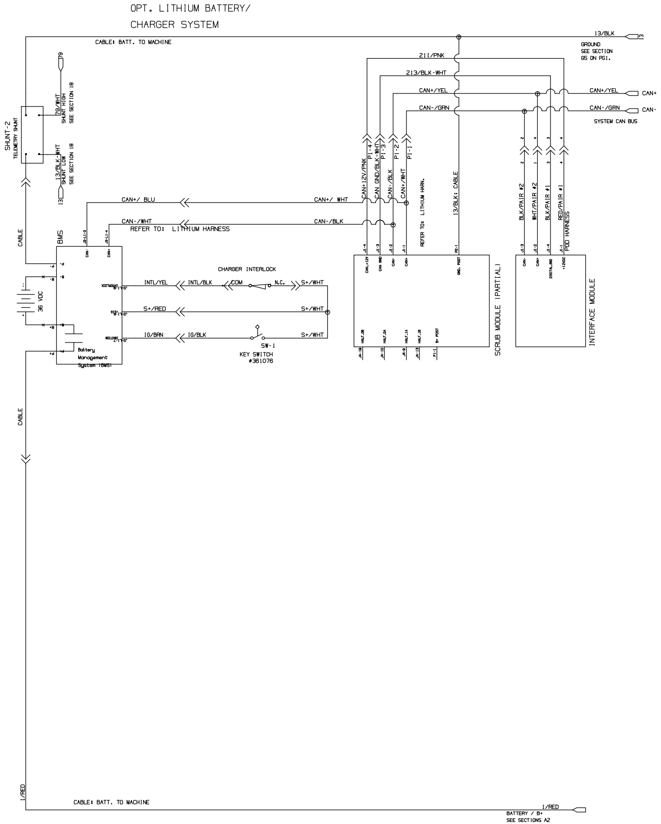
Fig. 35 – Electrical Schematic (1338– )
