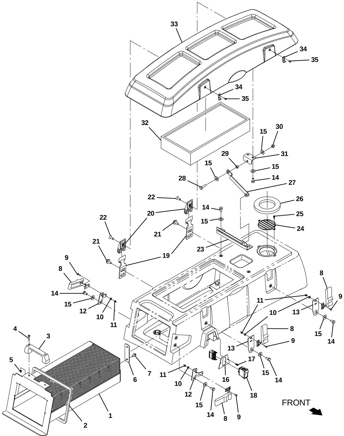
Fig. 52 – Dry Vacuum Debris Tray and Filter Group (1338– )
