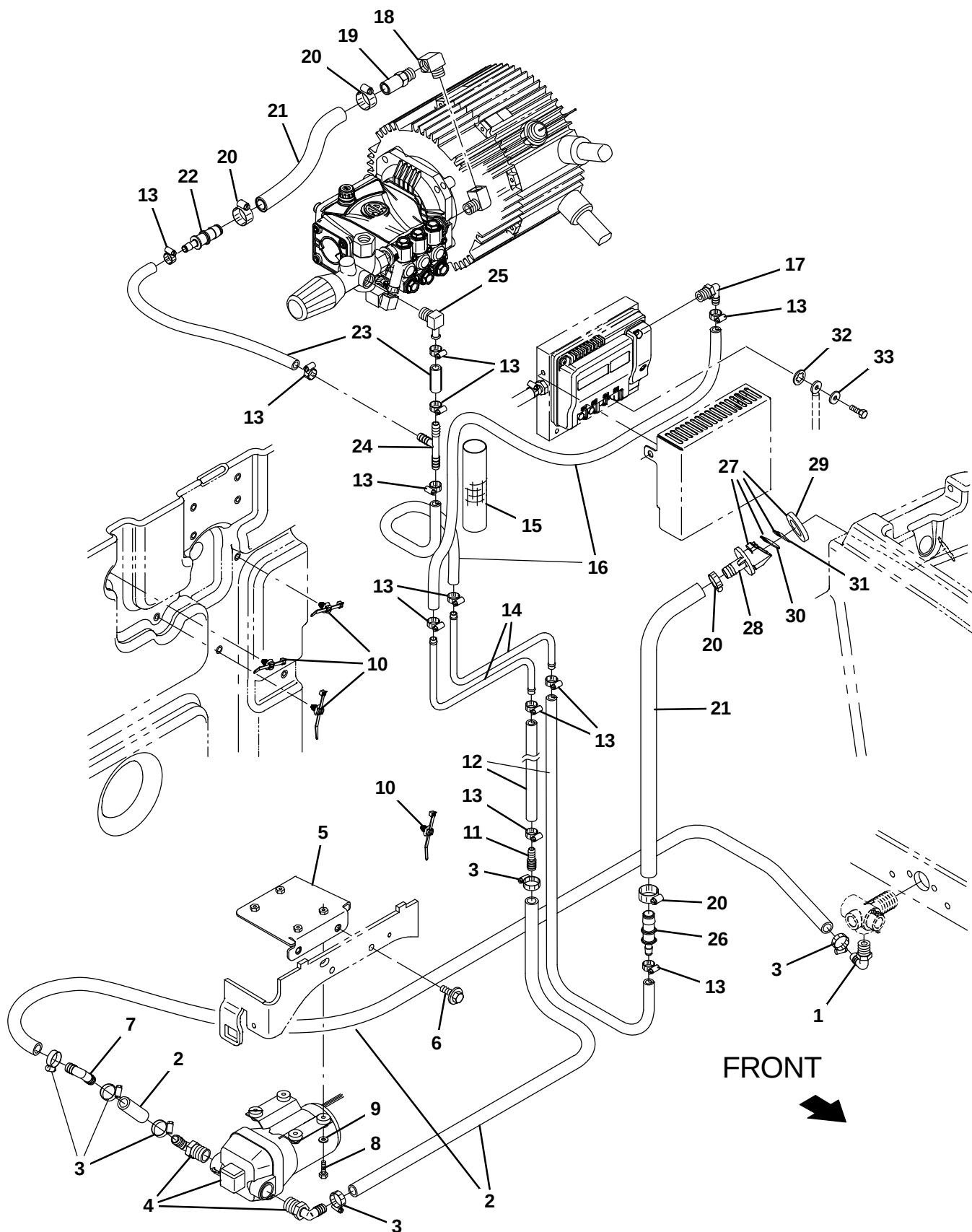
Fig. 45 – Pressure Washer Solution Supply Group (1200– )
