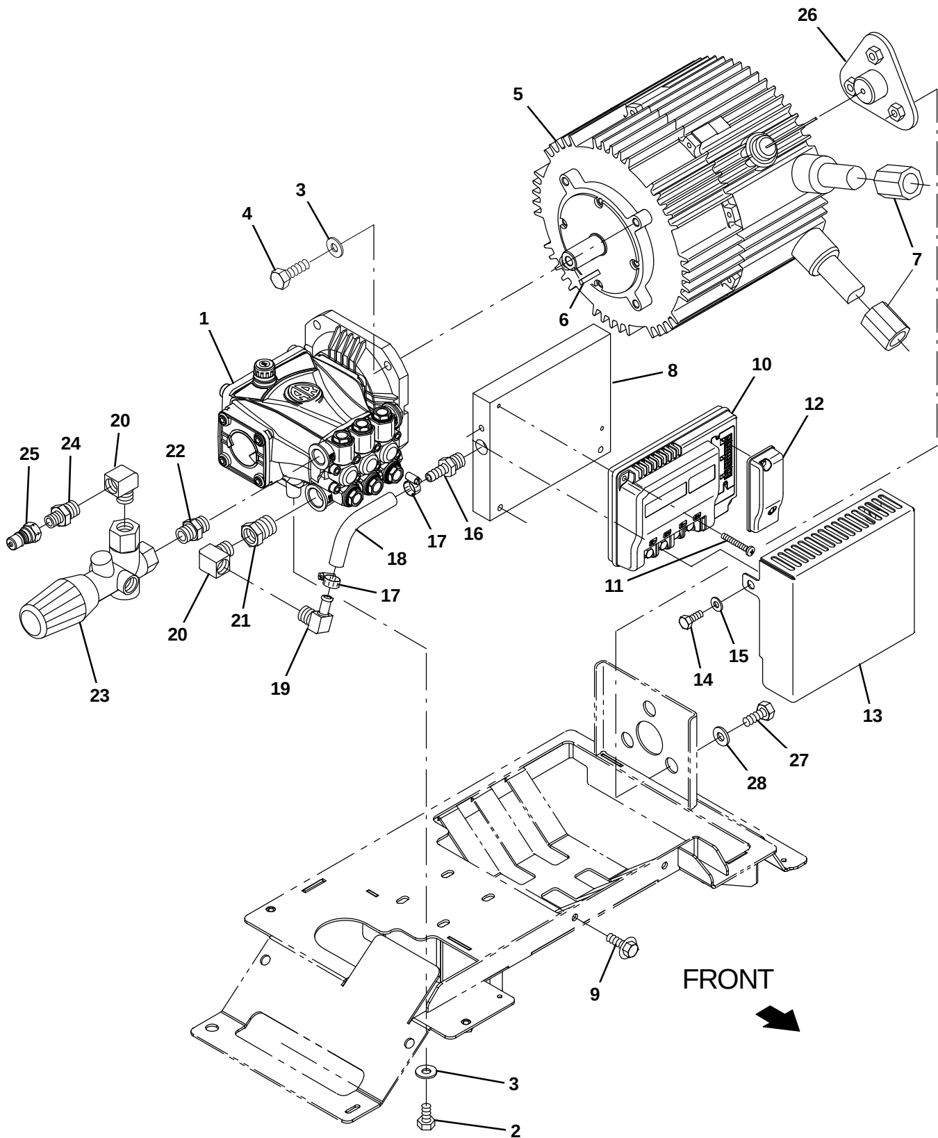
Fig. 46 – Pressure Washer Motor and Pump Group (1200– )
