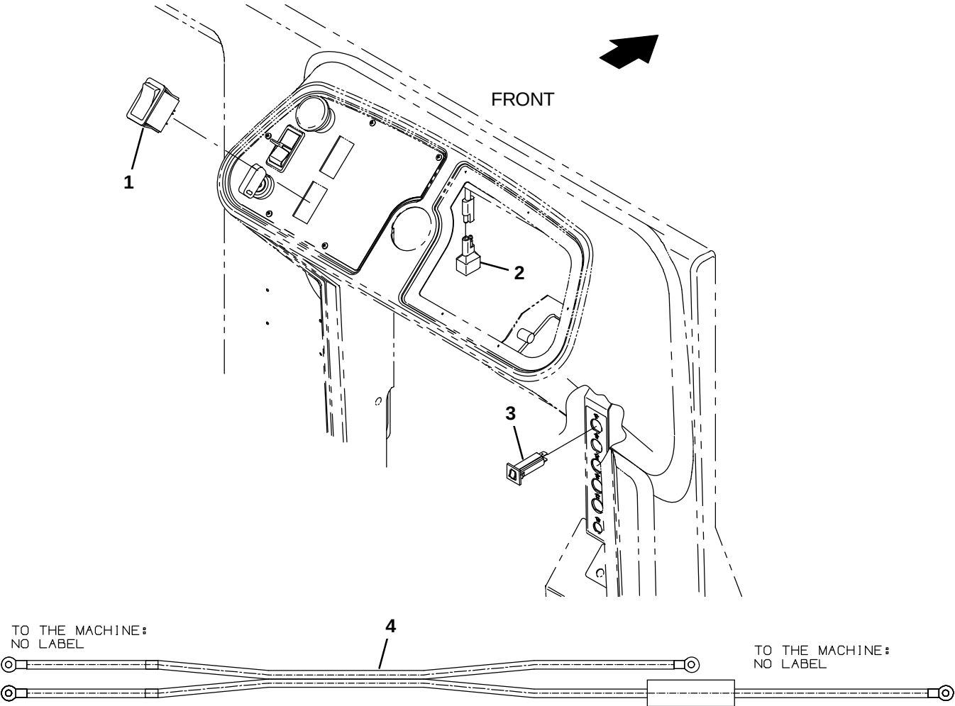
Fig. 47 – Pressure Washer Electrical Group (1200– )
