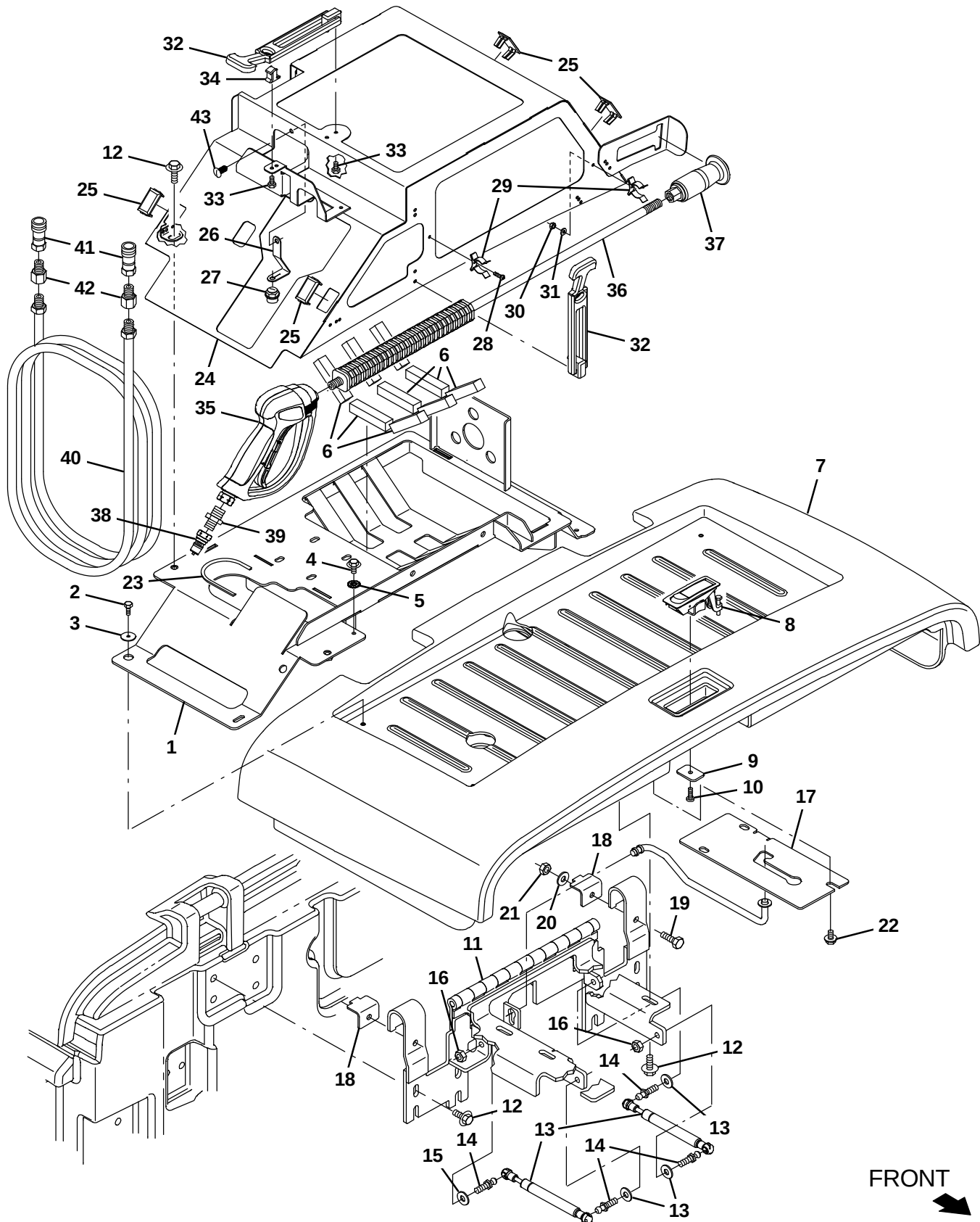
Fig. 44 – Pressure Washer Wand and Cover Group (1200– )
