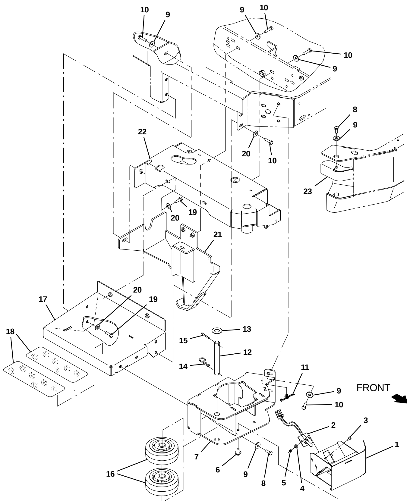
Fig. 53 – Dry Vacuum Nozzle Holder Group (1338– )
