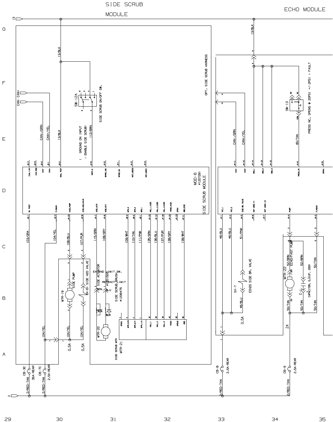
Fig. 33 – Electrical Schematic (0400–1199)
