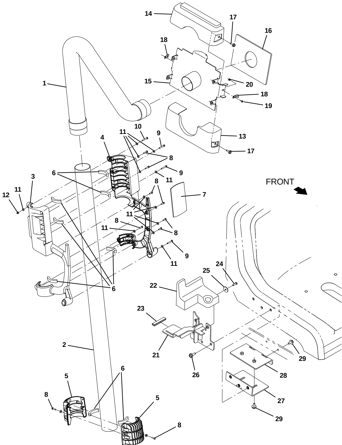
Fig. 49 – Dry Vacuum Wand Group (1338– )
