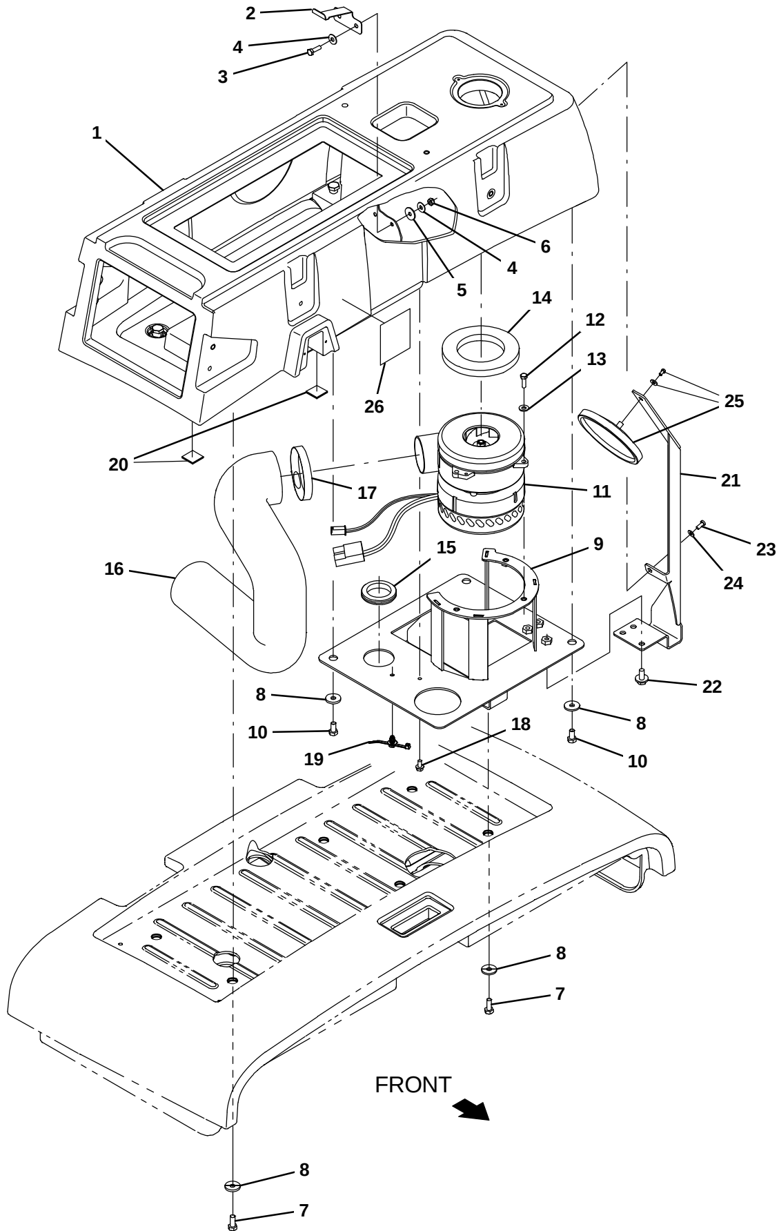
Fig. 51 – Dry Vacuum Fan and Housing Group (1338– )
