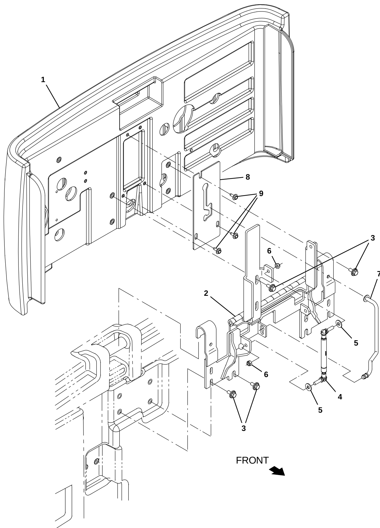
Fig. 50 – Dry Vacuum Rear Cover and Hinge Group (1338– )
