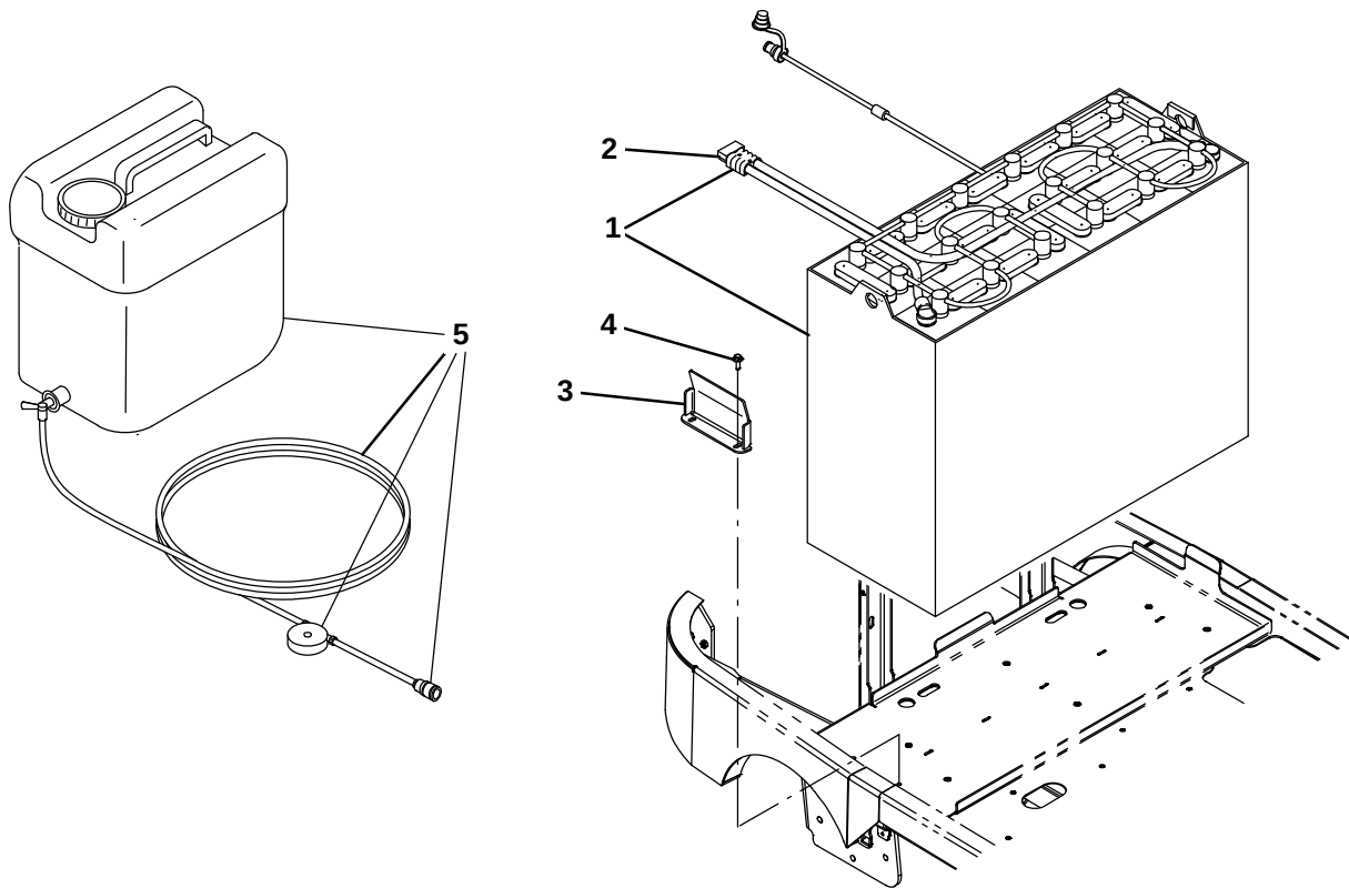
Fig. 40 – Battery Group
