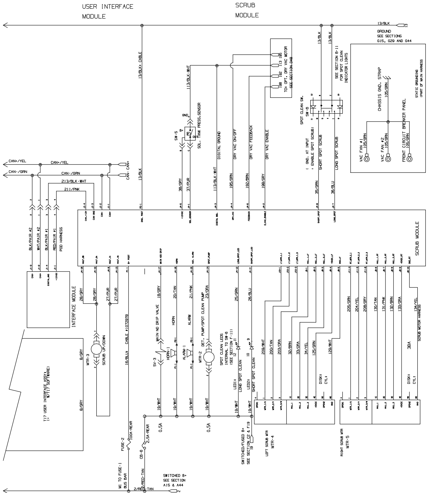
Fig. 35 – Electrical Schematic (1338– )
