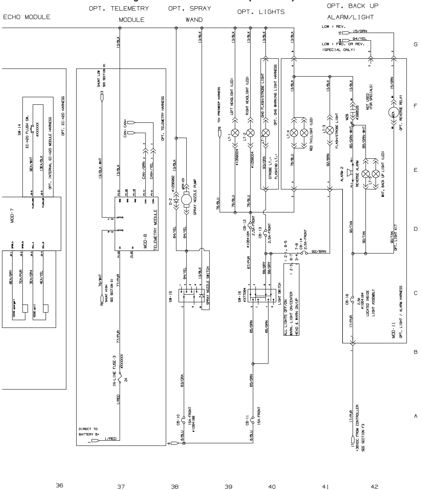
Fig. 33 – Electrical Schematic (0400-1199)
