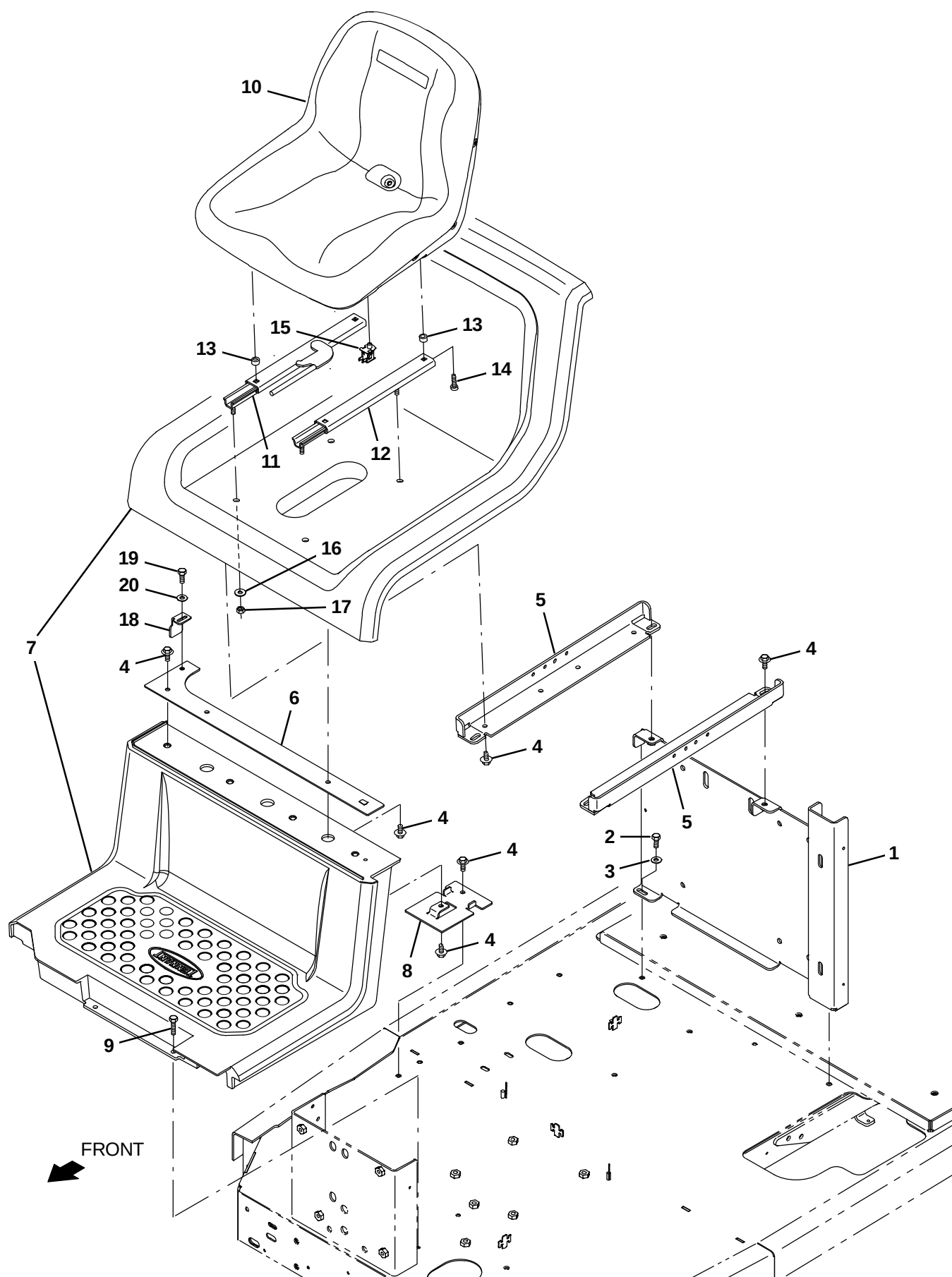
Fig. 8 – Seat Group
