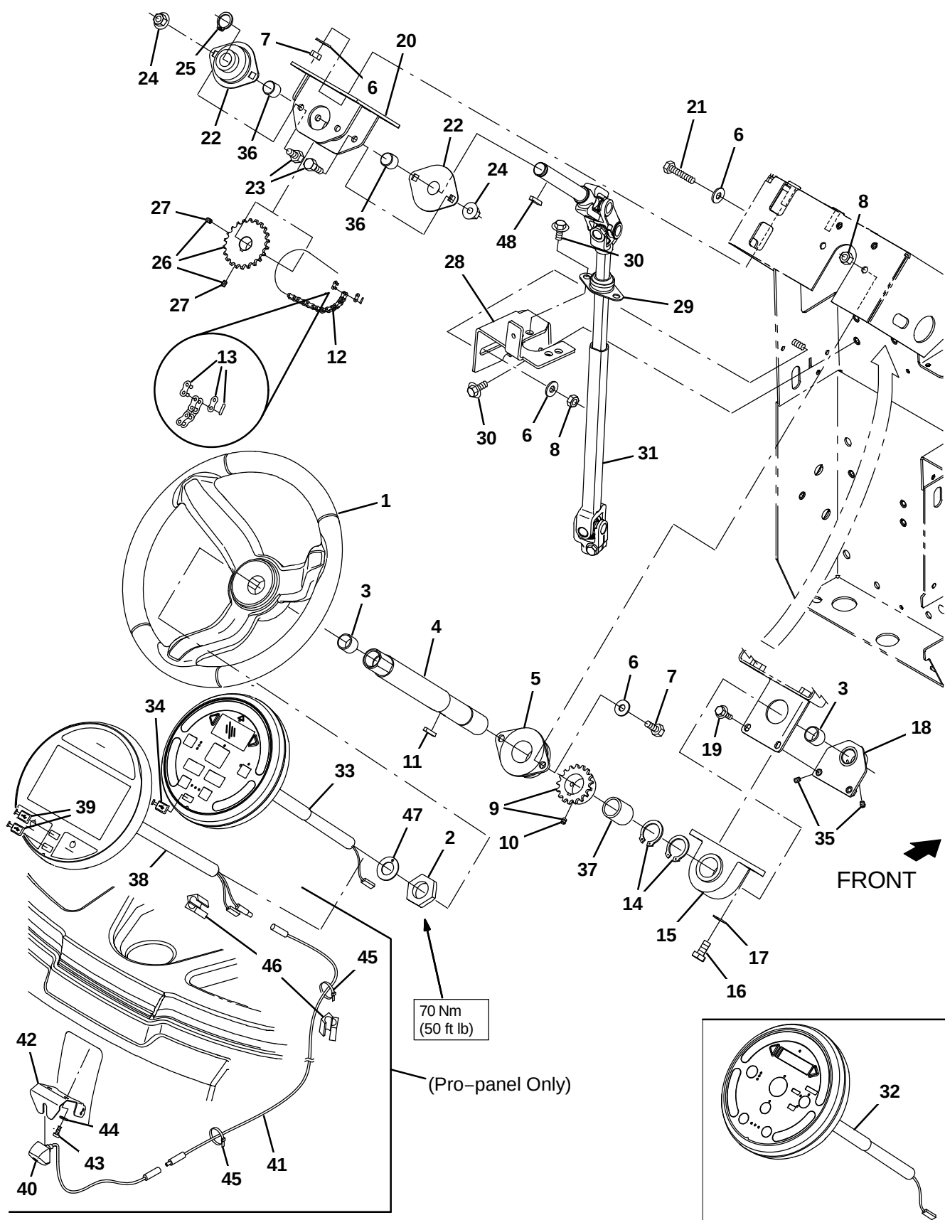
Fig. 5 – Steering Group
