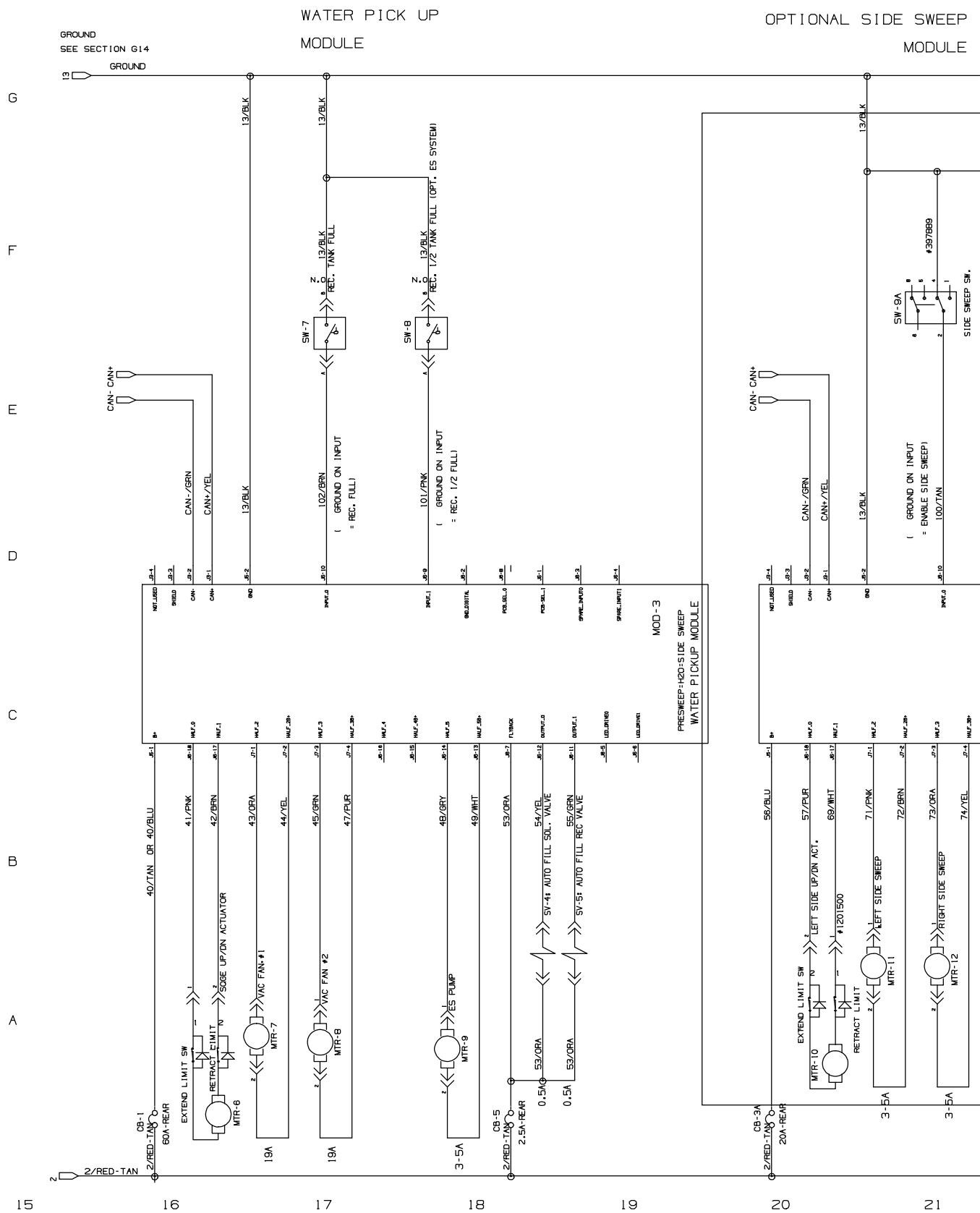
Fig. 32 – Electrical Schematic (0000–0399)
