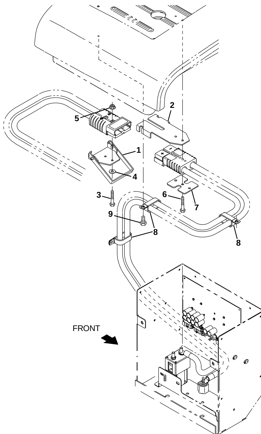
Fig. 55 – Battery Quick Disconnect Group (1200– )
