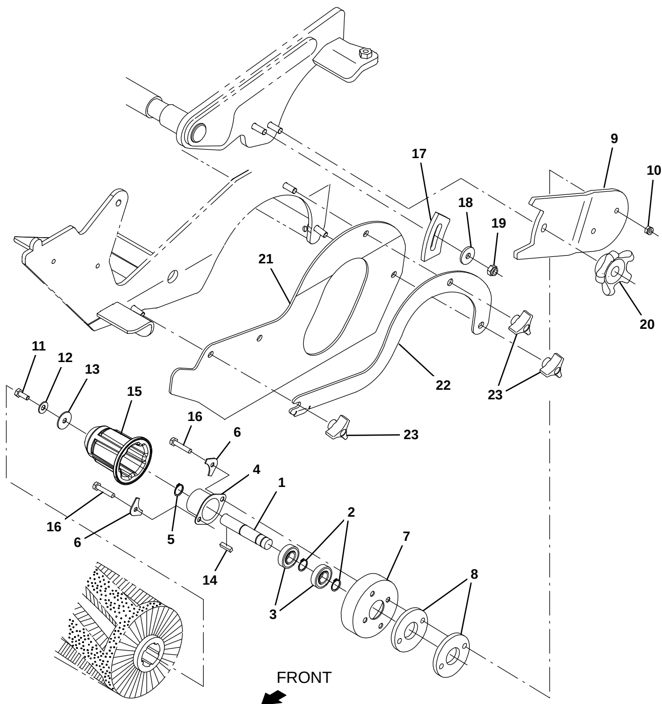
Fig. 23 – Pre-Sweep Brush Idler Group
