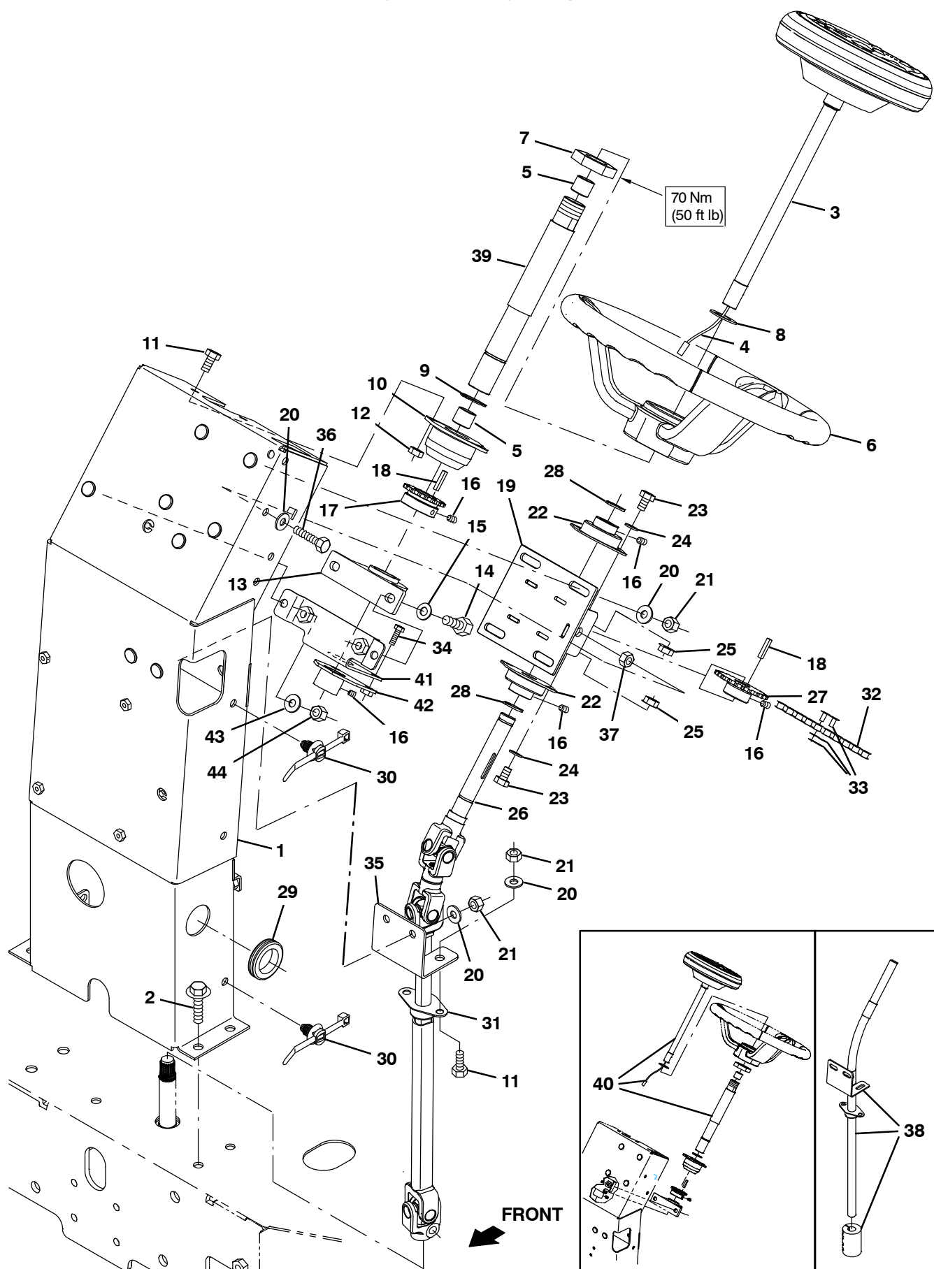
Fig. 5 – Steering Group
