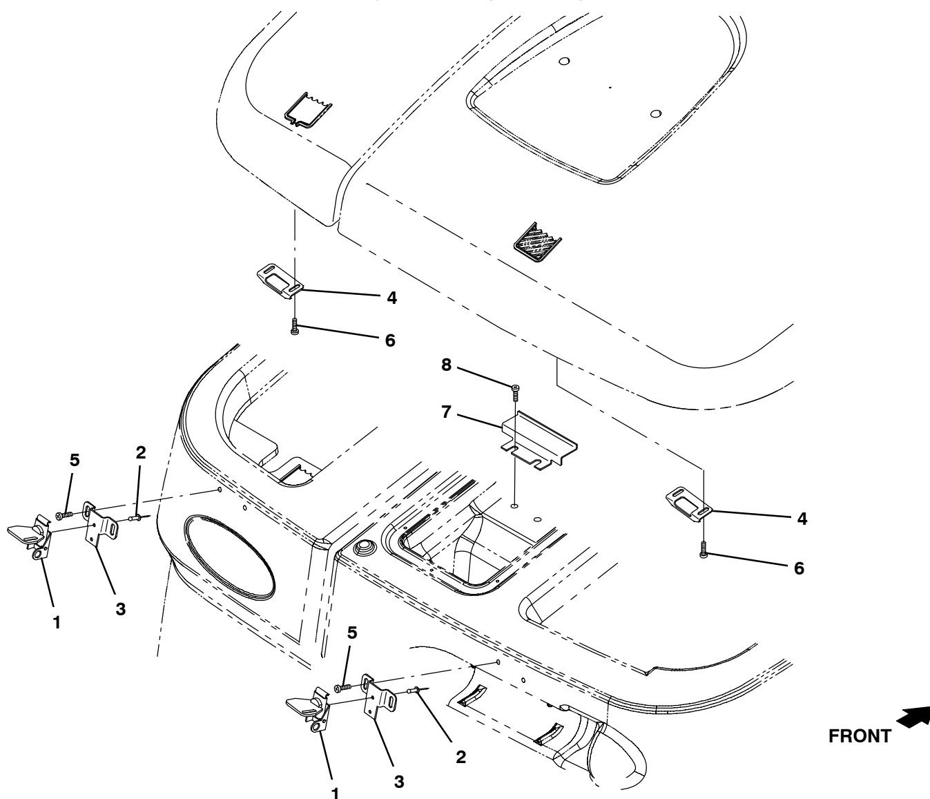
Fig. 25 – Transport Group
