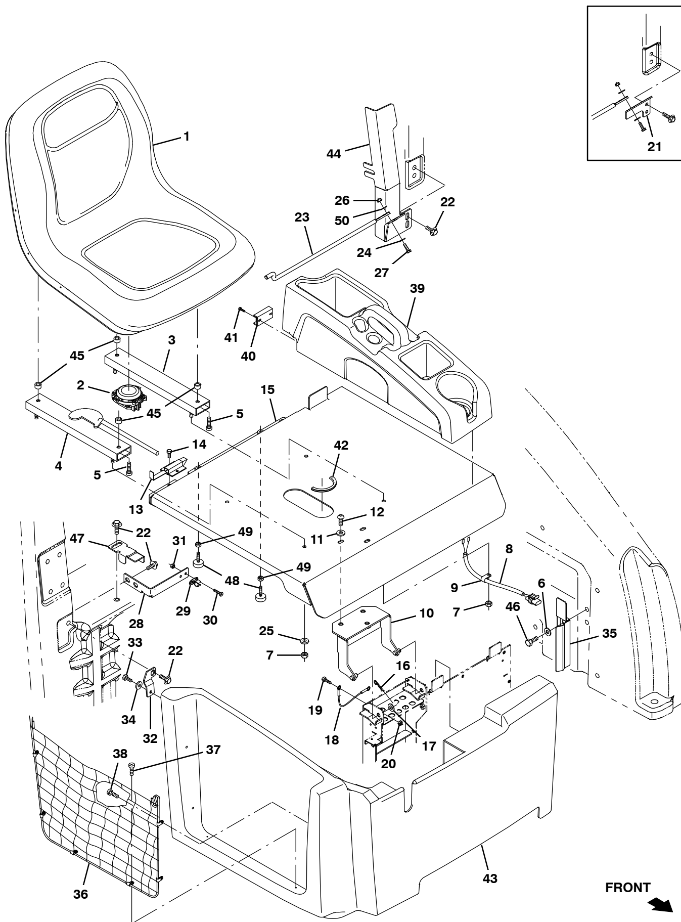
Fig. 4 – Seat Group
