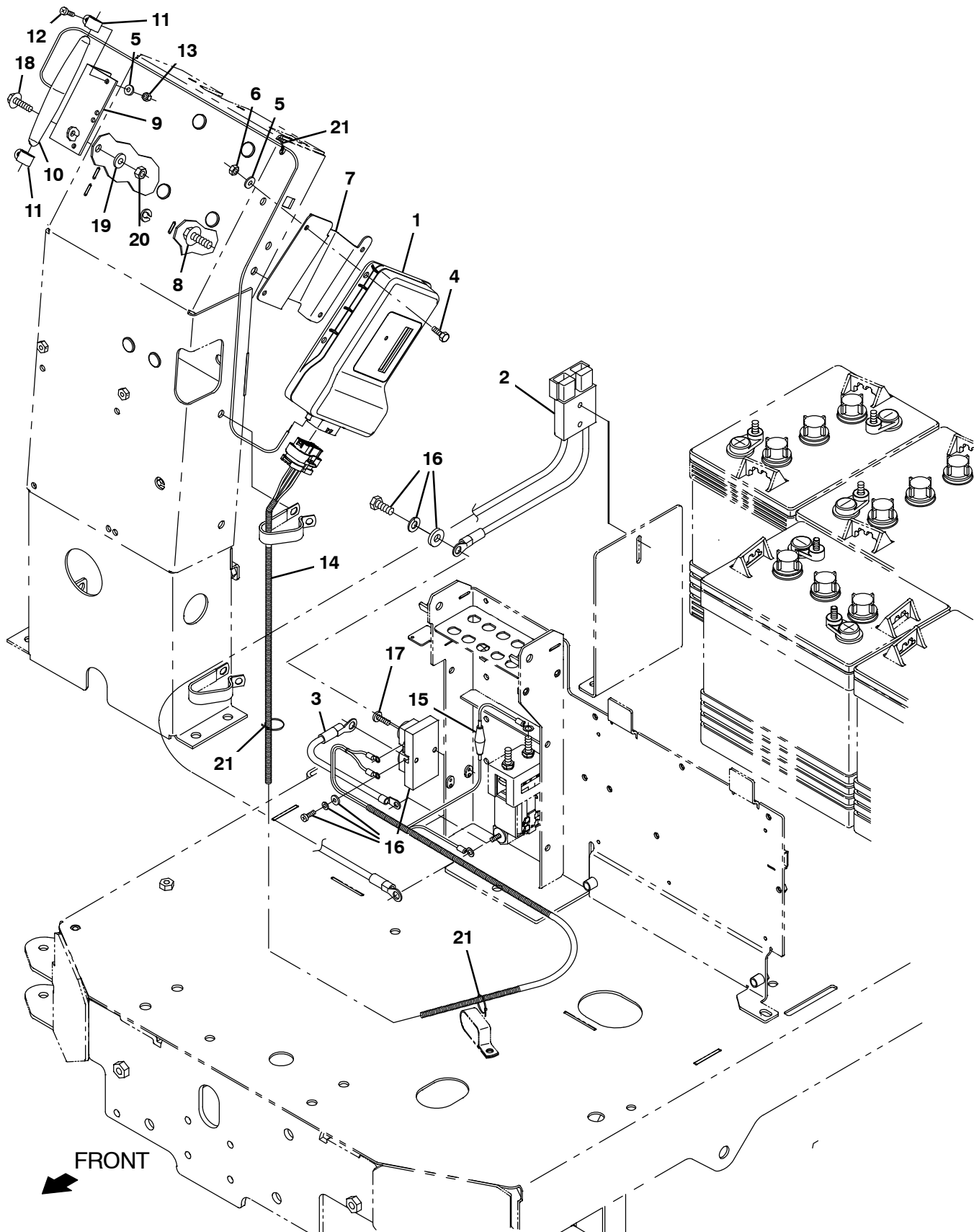
Fig. 31 – Telemetry Group
