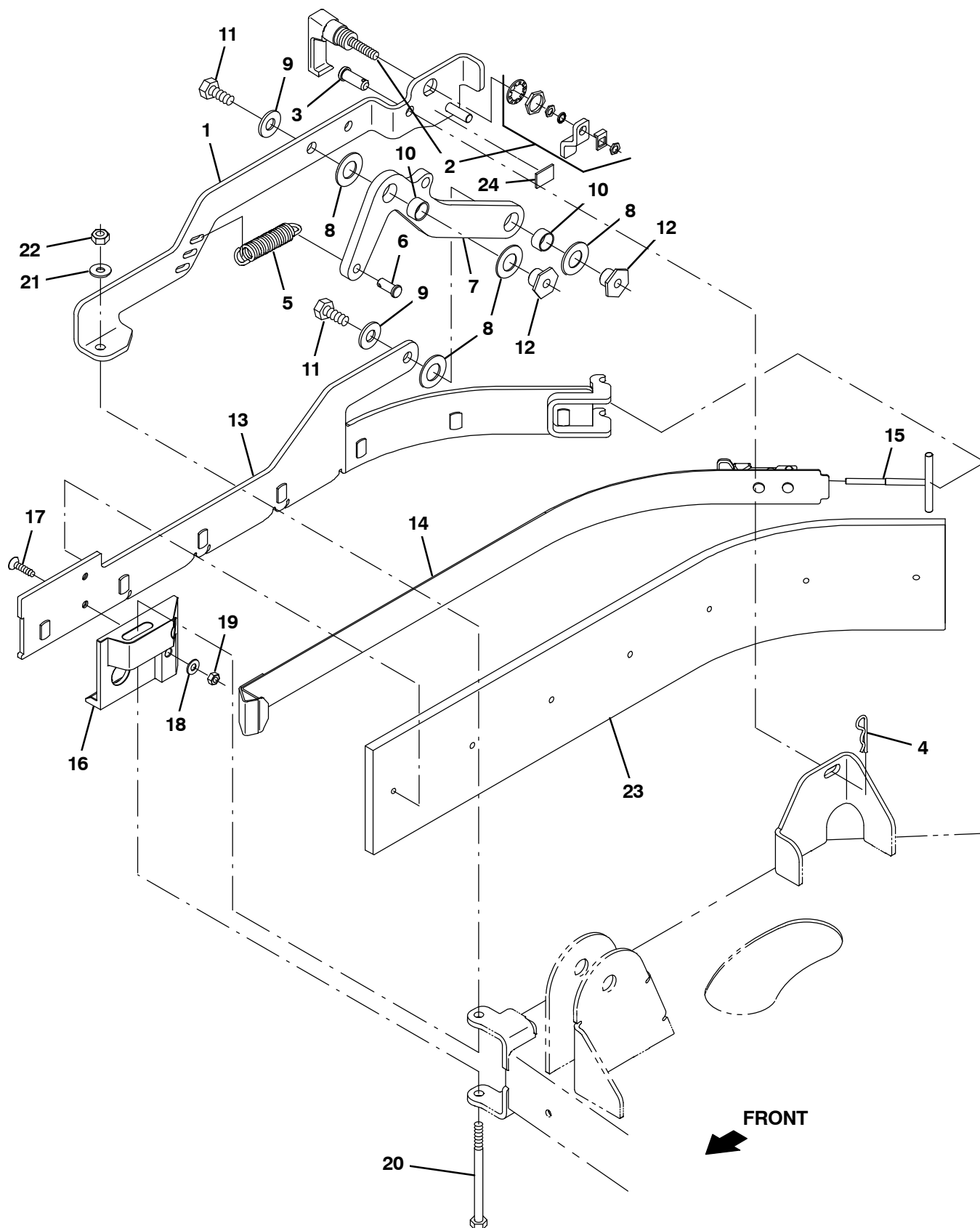
Fig. 14 – Scrub Head Side Squeegee Group, Right Hand
