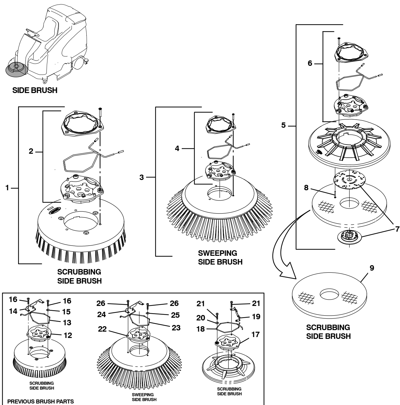
Fig. 2 – Replacement Brushes, Side Brush
