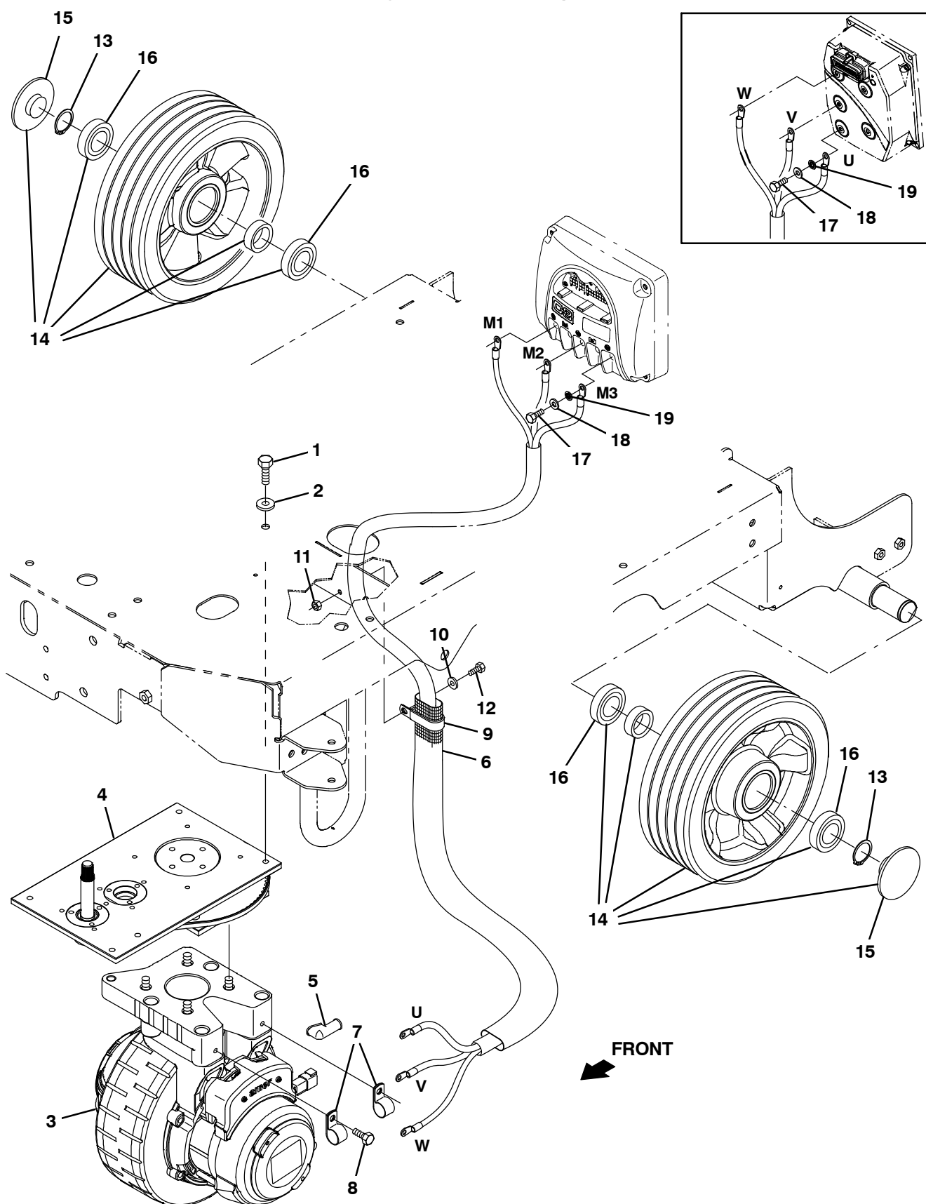
Fig. 9 – Wheels Group
