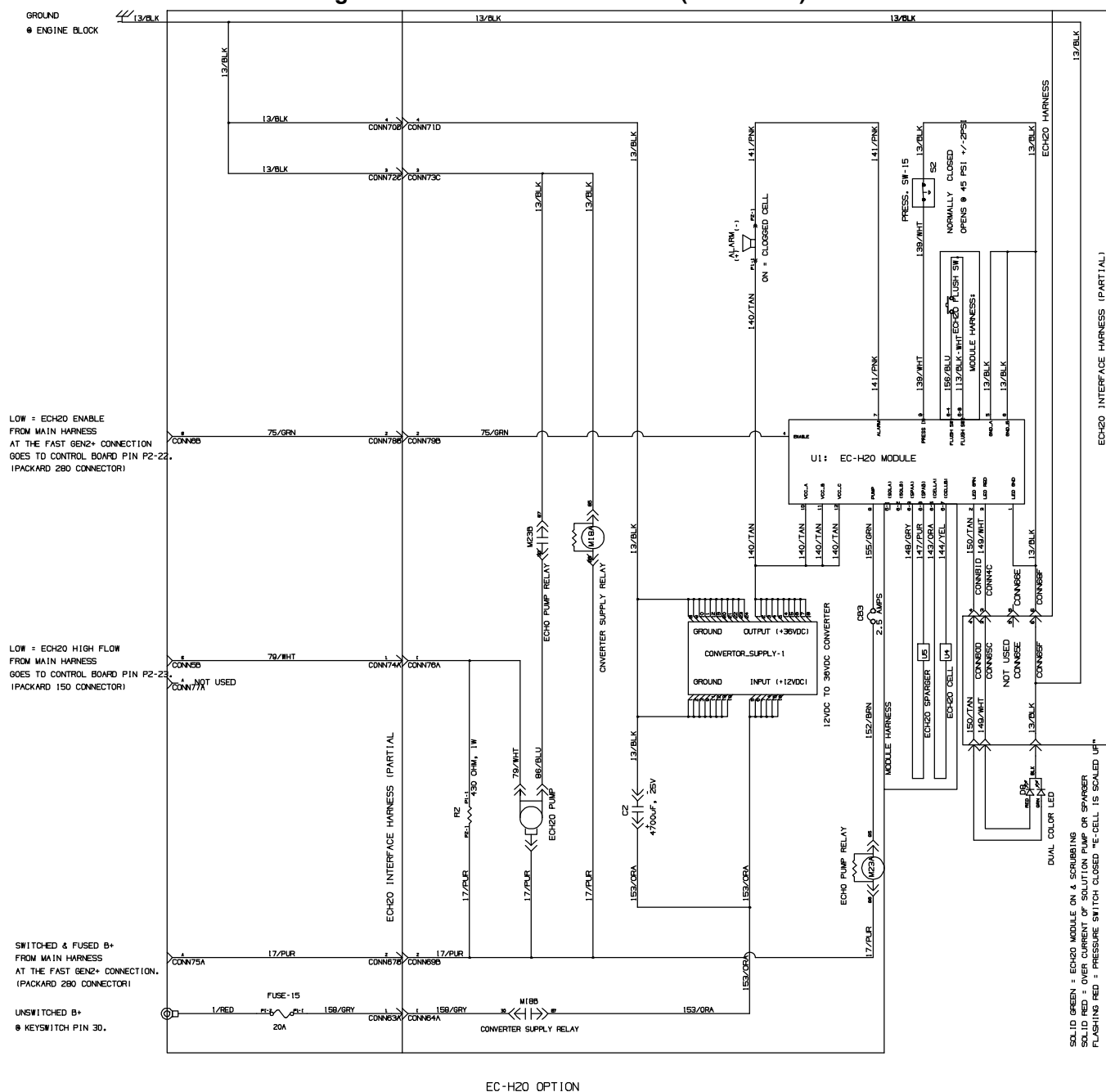
Fig. 85 – GM Electrical Schematic (0203–0499)
