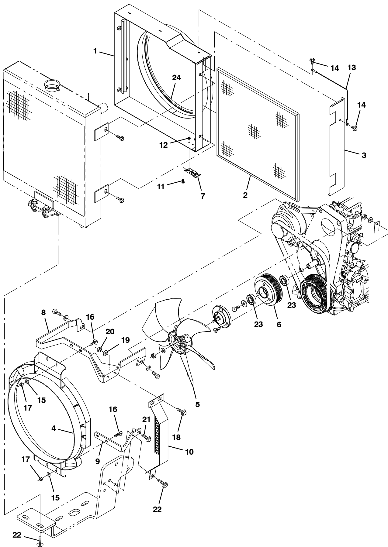
Fig. 40 – Engine Radiator Screen Kit (0203–0499)
