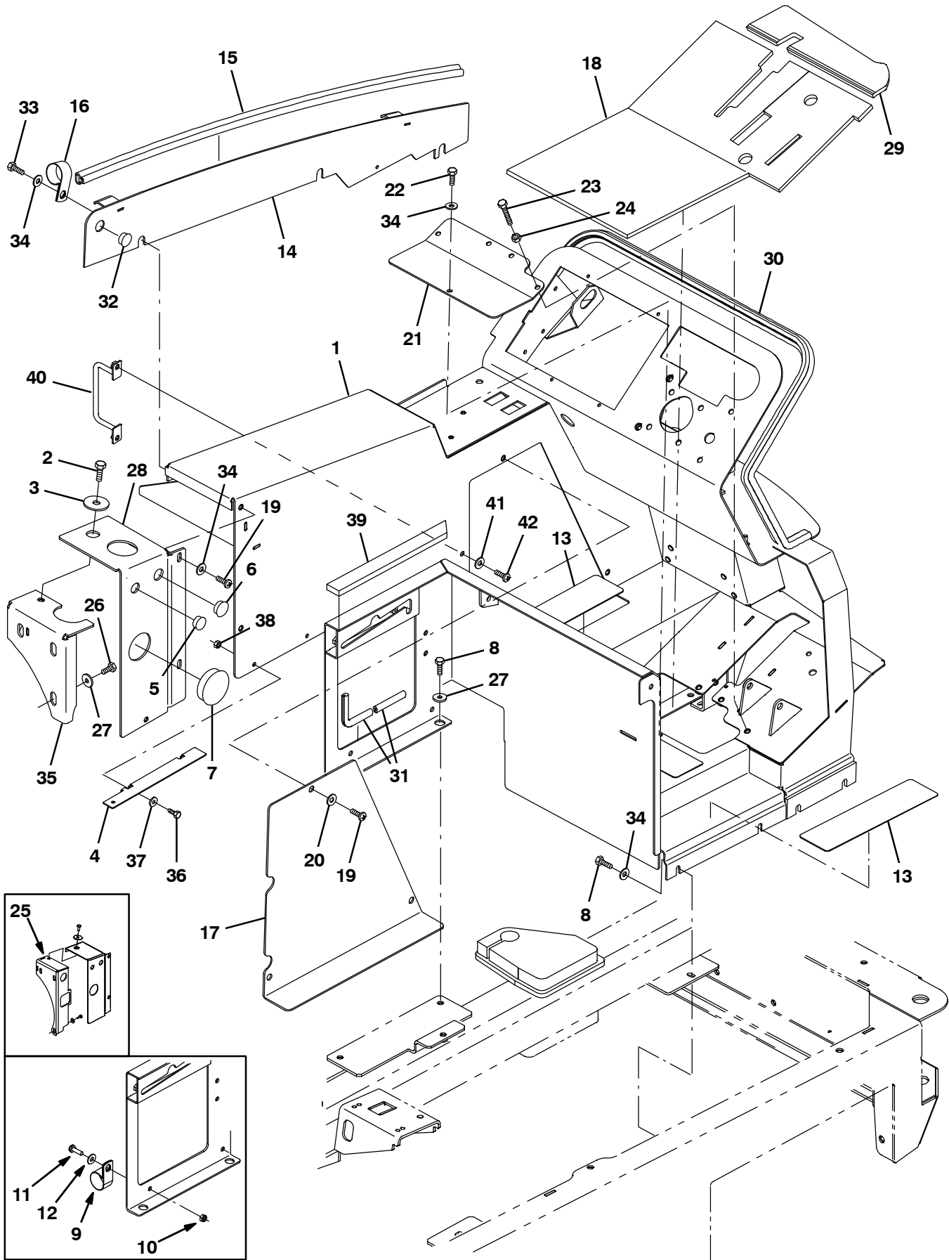
Fig. 4 – Operator Station
