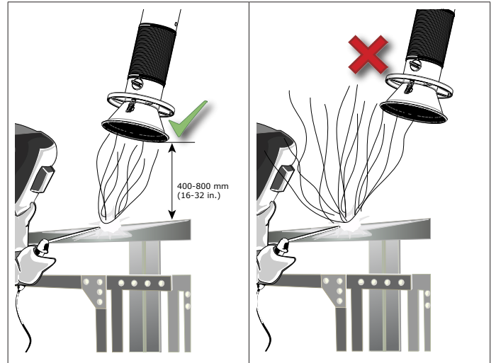
Fig. II Positioning of the extraction arm
