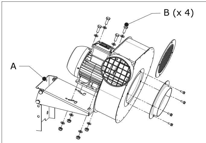
Fig. 4.2 Installing the fan on an MB-FUA-C1/C2
