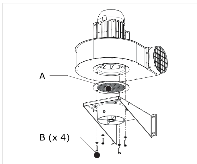
Fig. 4.5 Installing the fan directly on an arm
